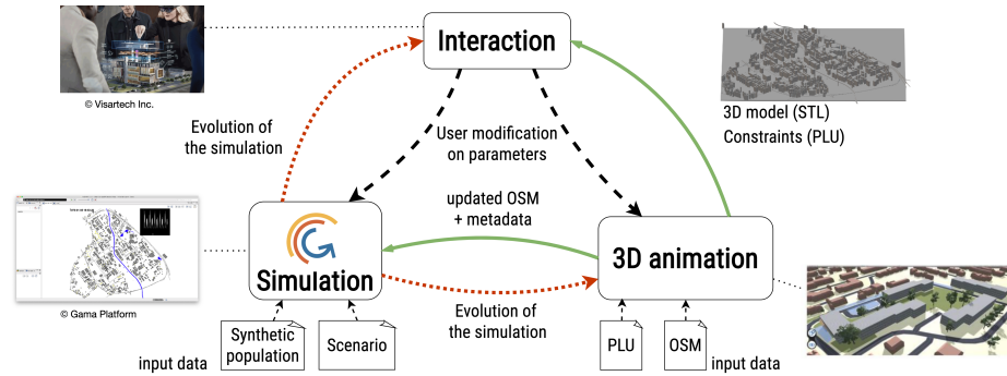
Fig. 1. Workflow of our phigital simulation approach. ( Interaction will use Hololens by Microsoft, image credit: https://www.visartech.com/blog/ )
