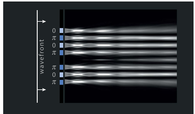
Figure 6. Calculation of the transmitted light intensity after a 0 – π chessboard grating, for a planar incoming light wavefront at normal incidence, where one hole of the grating is blocked. A self-healing of the beam is evidenced, showing the limitation of the shadowing picture.
