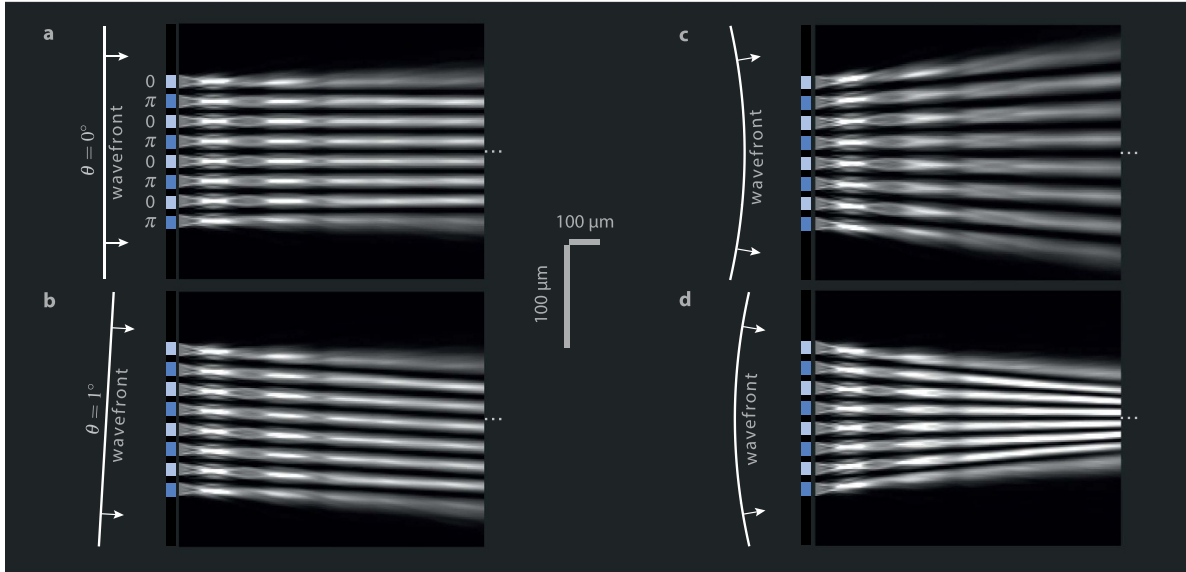
Figure 5. The QLSI principle understood as a shadowing effect. (a) Calculation of the transmitted light intensity after a 0 – π chessboard grating, for a planar incoming light wavefront at normal incidence. For the sake of simplicity, the square grating contains 4 × 4 unit cells. A diffraction-less shadowing effect is observed. (b) Same calculation when the wavefront is tilted by an angle of 1°, producing a lateral shift of the shadow according to this same angle. (c) Simulation of transmitted light when the wavefront is convex, producing a spreading of the shadow. (d) Simulation of transmitted light when the wavefront is concave, producing a shrinking of the shadow.
