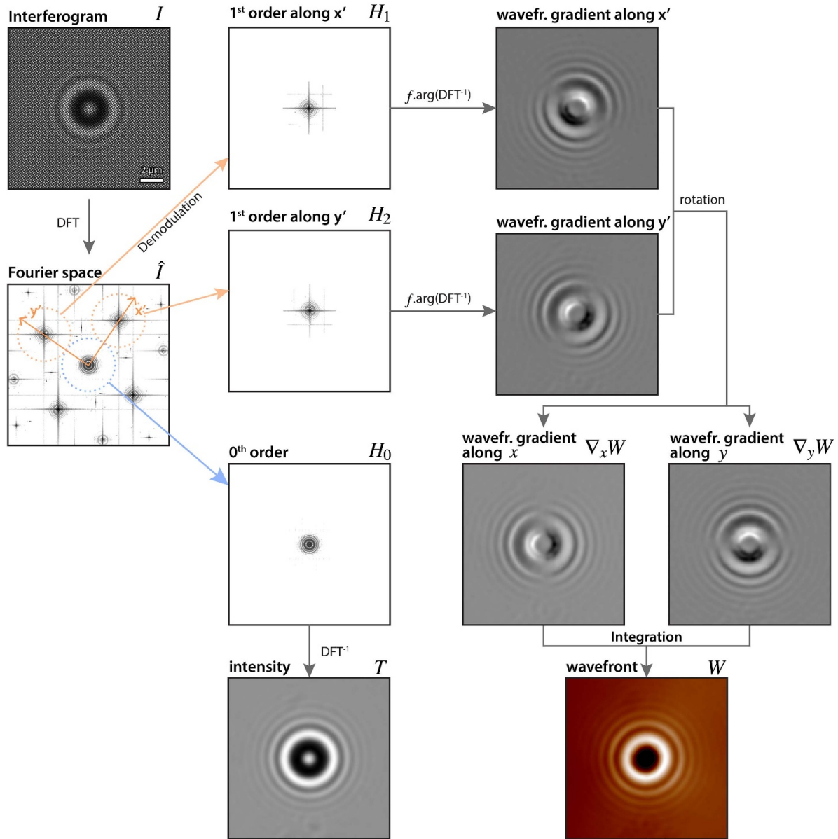
Figure 7. Summary schematic of the full intensity and wavefront retrieval algorithm, illustrated with the image of a 2 μm dielectric bead.
