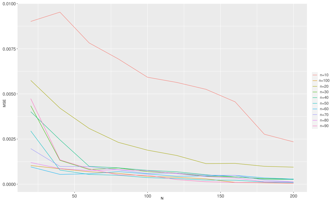
FIGURE 5. MSE of the looCV estimator with respect to N and n for Model 1.
