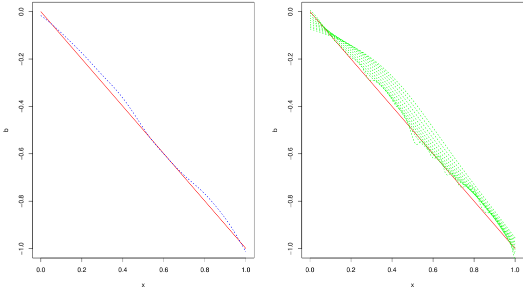
FIGURE 2. LooCV NW estimation for Model 2 (hyperbolic diffusion process), \hat{h} = 0.04 .
