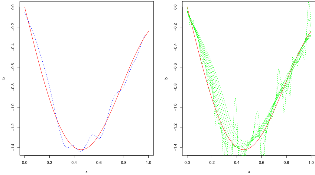
FIGURE 4. LooCV NW estimation for Model 4, \hat{h} = 0.06 .
