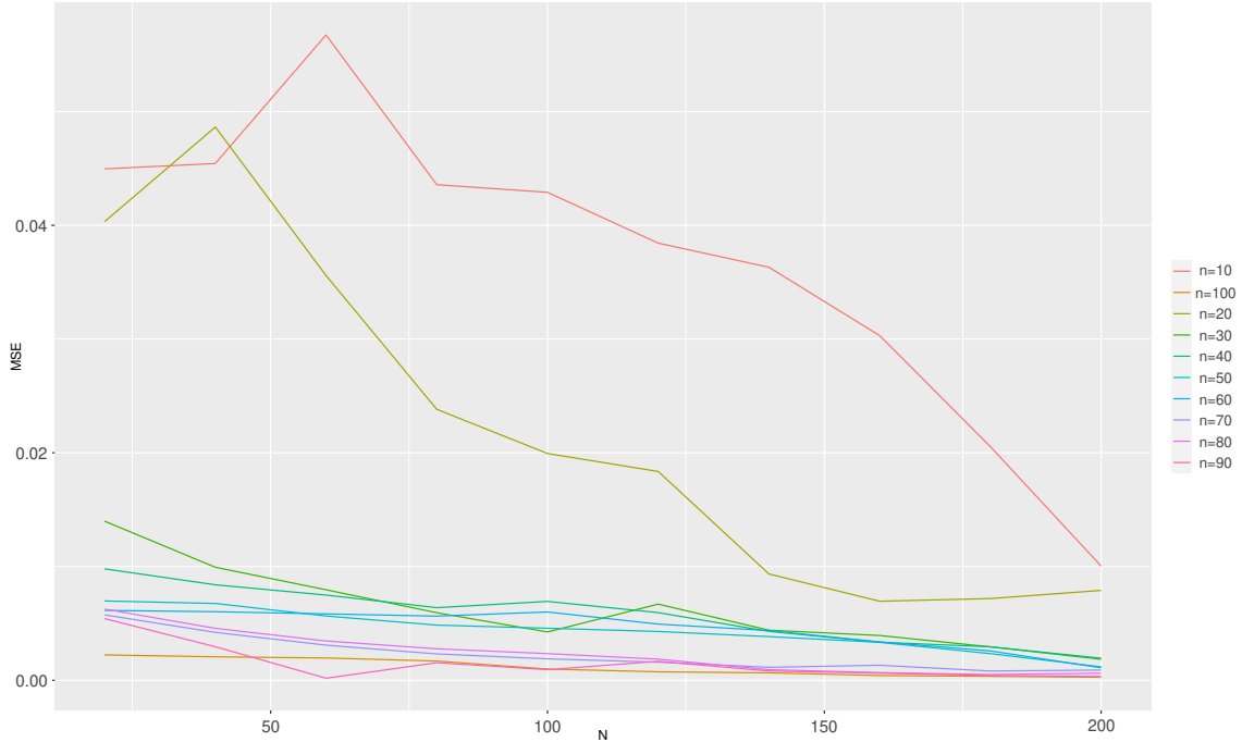
FIGURE 6. MSE of the looCV estimator with respect to N and n for Model 3.
