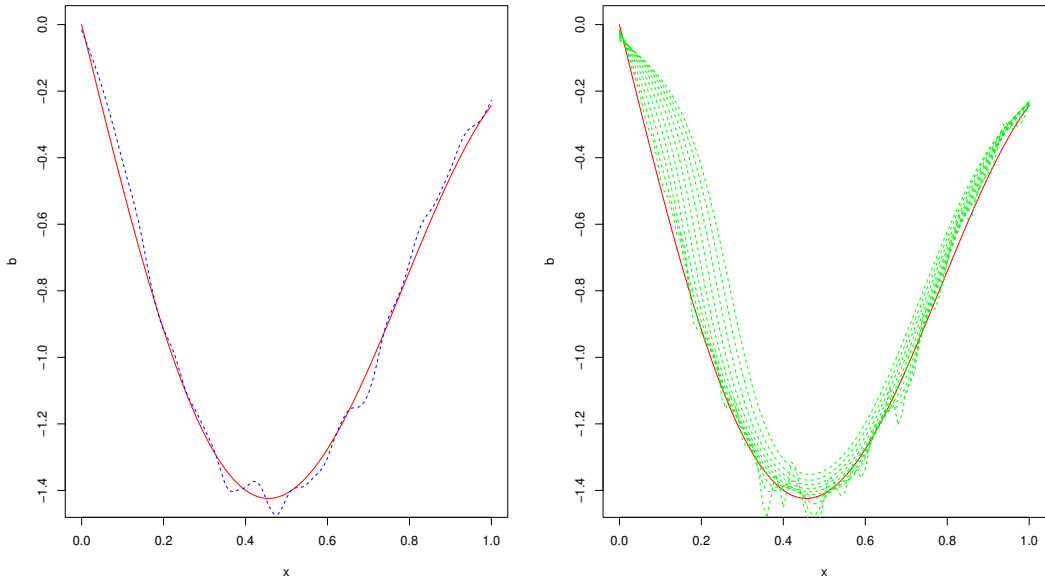
FIGURE 3. LooCV NW estimation for Model 3, \hat{h} = 0.02 .
