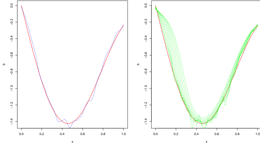
FIGURE 3. LooCV NW estimation for Model 3, \hat{h} = 0.02 .
