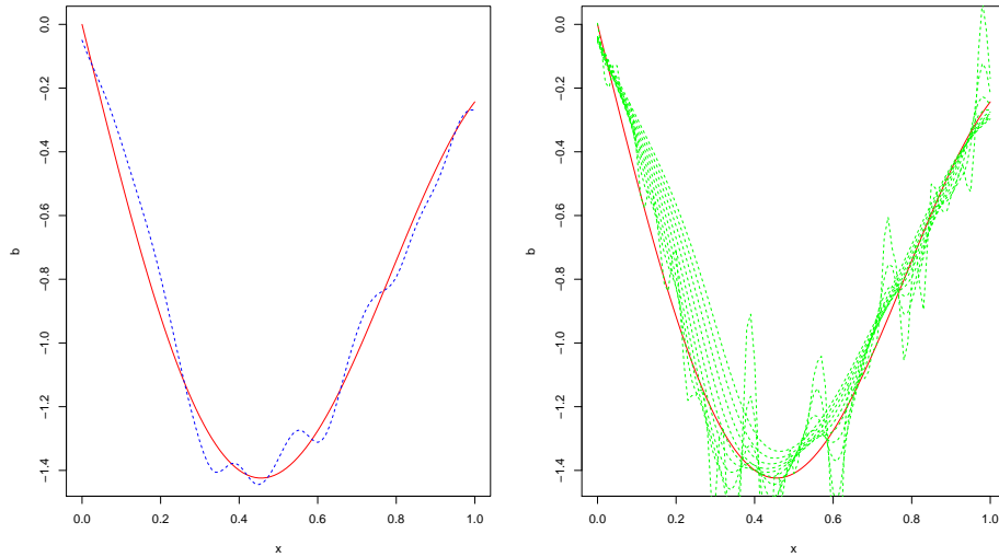
FIGURE 4. LooCV NW estimation for Model 4, \hat{h} = 0.06 .
