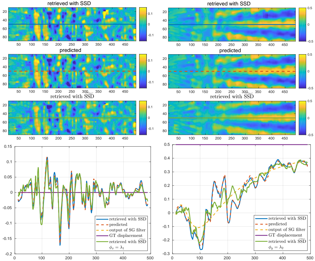
Figure 22: Large speckle, 19 \times 19 subset \Omega , zero-order shape functions, and displacement estimation (along x - on the left and y -axis on the right) with the 2D\text{-SSD} criterion.
