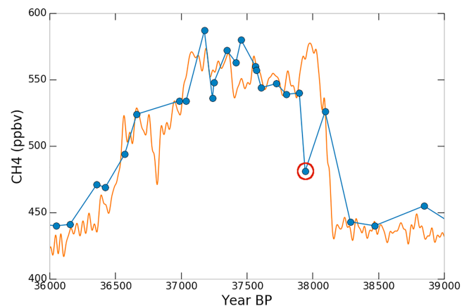
Figure 7. Discrete EDC methane record (blue) and continuous WDC methane record (orange). The WDC record was put on the GICC05 timescale and then shifted by 250 years to improve matching. We suggest that the circled point corresponds to a layered trapping artifact.
