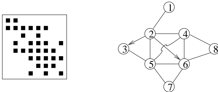
Figure 29.1: Sparsity pattern (left) and adjacency graph (right) of a 8 \times 8 sparse matrix.
