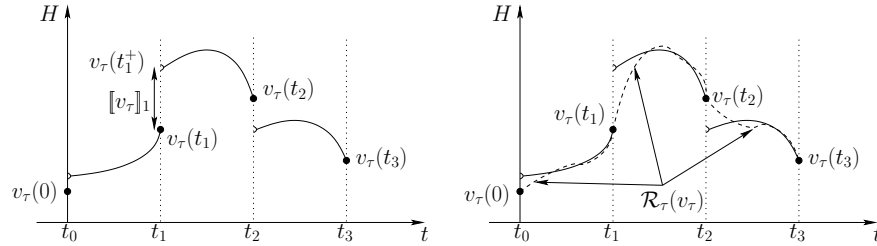
Figure 69.1: Example of time-discrete function v_\tau \in P_k^b(\bar{J}_\tau; H) (left panel) and its time reconstruction \mathcal{R}_\tau(v_\tau) \in P_{k+1}^g(\bar{J}_\tau; H) (right panel, bold dashed curve, see Definition 69.5).
