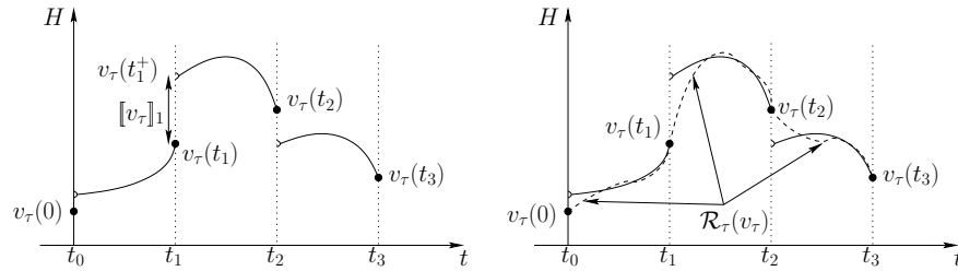
Figure 69.1: Example of time-discrete function v_\tau \in P_k^b(\overline{J}_\tau; H) (left panel) and its time reconstruction \mathcal{R}_\tau(v_\tau) \in P_{k+1}^g(\overline{J}_\tau; H) (right panel, bold dashed curve, see Definition 69.5).
