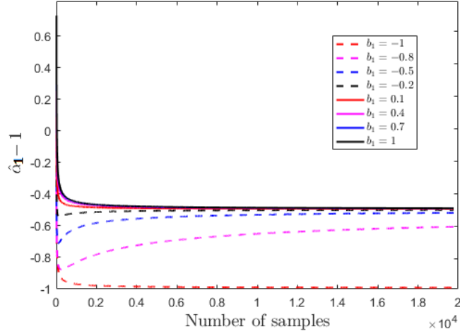
Figure 7: Abacus based on the DFA giving \hat{\alpha}_1 - 1 for different values of M and different MA parameters
