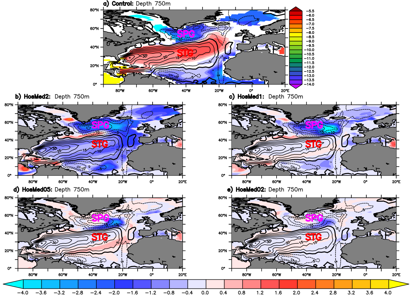
Figure 7. a) Horizontal maps of \epsilon_{Nd} distribution at 750 m depth in the North Atlantic basin. b), c), d) and e) \epsilon_{Nd} anomalies between control simulation and HosMed2, HosMed1, HosMed05 and HosMed02, respectively. Shown in contour the mean of the barotropic stream function in the control simulation averaged over 1000 years SPG (Subpolar Gyre), STG (subtropical gyre). We only show the differences significant at the 95% level following a student t-test.
