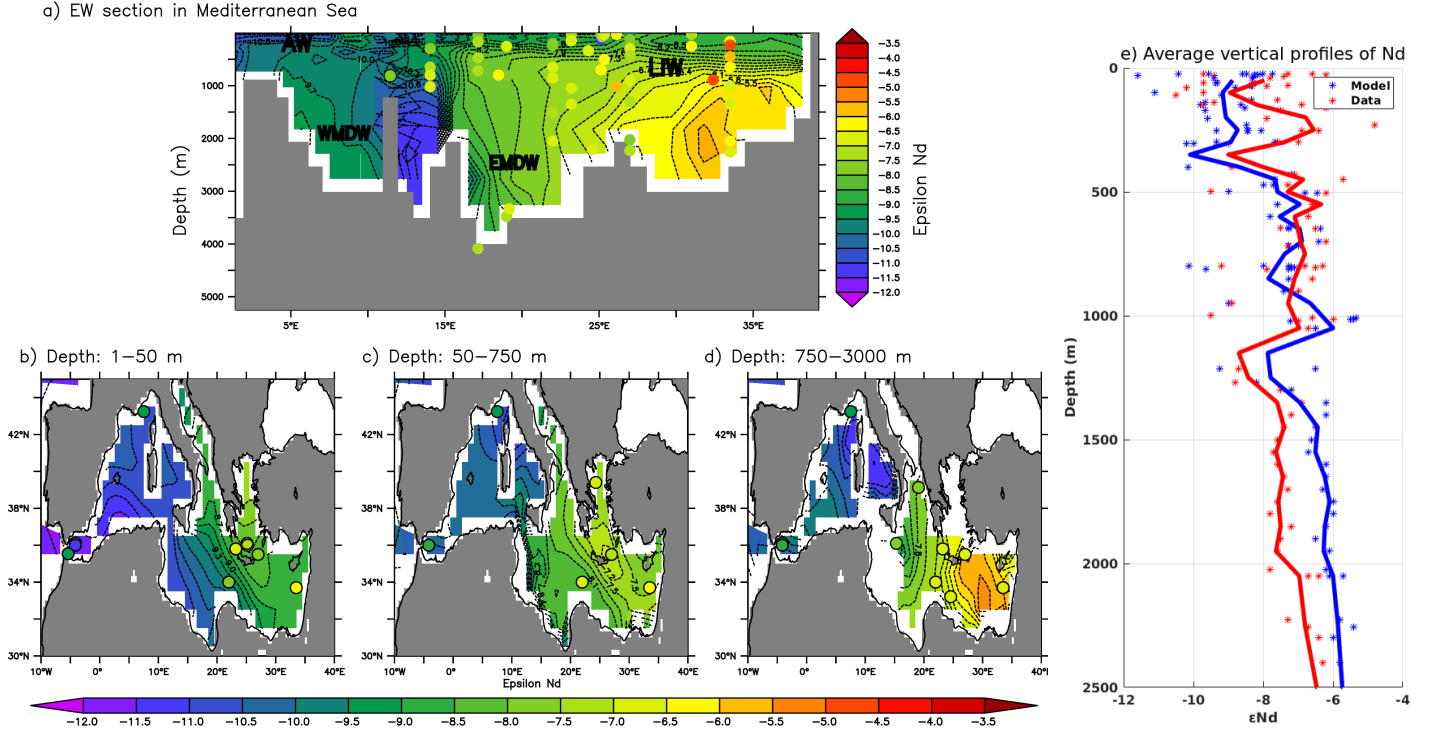
Figure 1. Model-data comparison of \epsilon_{\text{Nd}} for the Mediterranean Sea from control simulation (averaged over last 100 years). Upper line East-West section (a). Lower panel: horizontal maps for surface waters (b), intermediate waters (c), and deep waters (d). Color-filled dots represent in situ observations from Tachikawa et al. (2004), Vance et al. (2004) and Henry et al. (1994). Both use the same colour scale. LIW (Levantine intermediate water), AW (Atlantic Waters), WMDW (Western Mediterranean Deep Water) EMDW (Eastern Mediterranean Deep Water) appears in panel a). e) Comparison of average vertical profiles of Nd isotopic signature ( \epsilon_{\text{Nd}} ) from control run in the whole Mediterranean Sea. Model results are in blue, while red indicates the in situ data from Tachikawa et al. (2004), Vance et al. (2004) and Henry et al. (1994).
