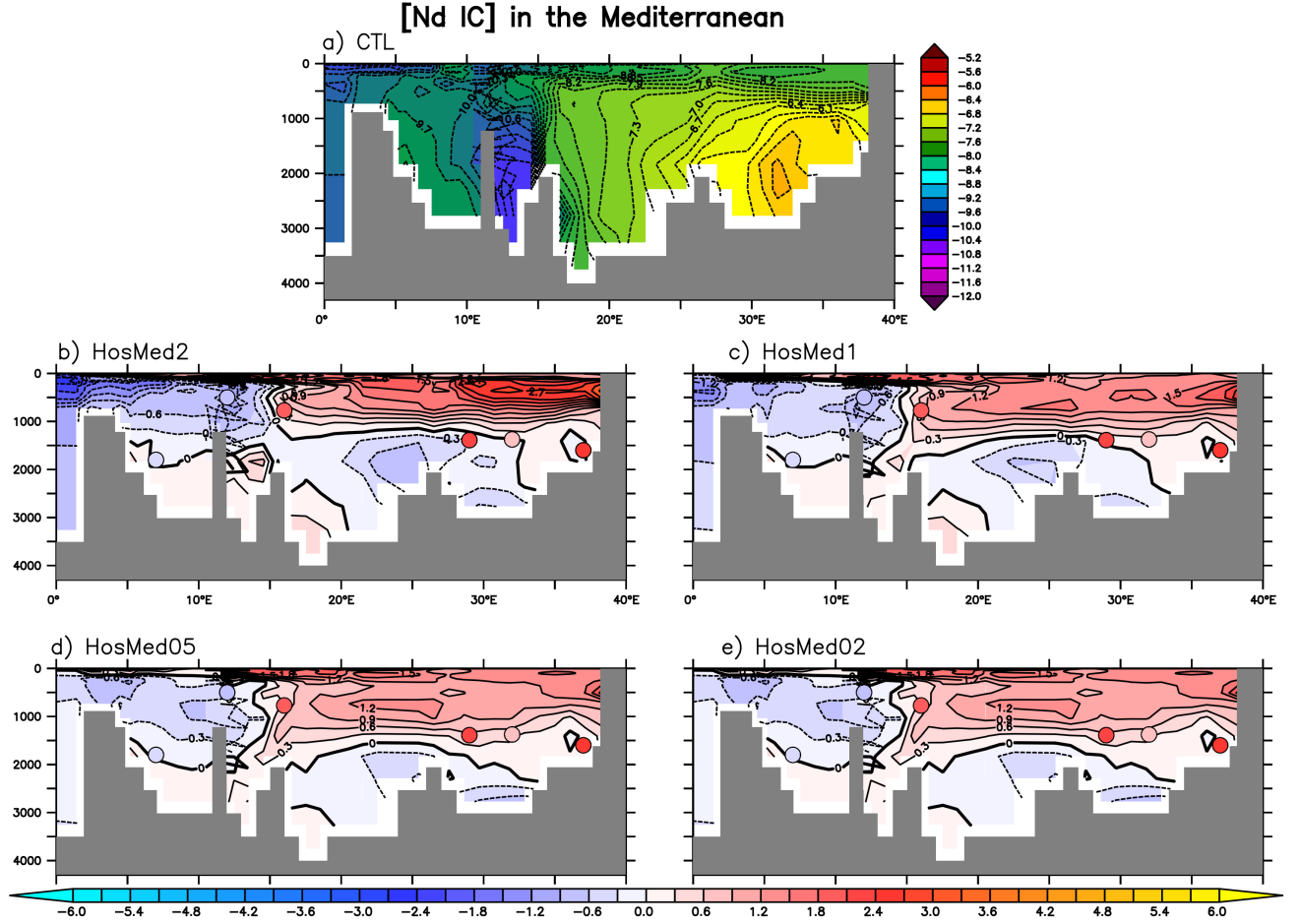
Figure A2. a) Vertical sections along an east-west transect in the Mediterranean Sea. b), c), d) and e) \epsilon_{\text{Nd}} anomalies between control simulation and HosMed2, HosMed1, HosMed05 and HosMed02 respectively. Dots represents the \epsilon_{\text{Nd}} signal recorded in Alboran Sea (Jiménez-Espejo et al., 2015), Sardinia Chanel (Dubois-Dauphin et al., 2017), Sicily Strait, Levantine Basin (Cornuault et al., 2018), and from Duhamel et al. (2020) for the west-Levantine basin. The data are shown in comparison to modern \epsilon_{\text{Nd}} values.
