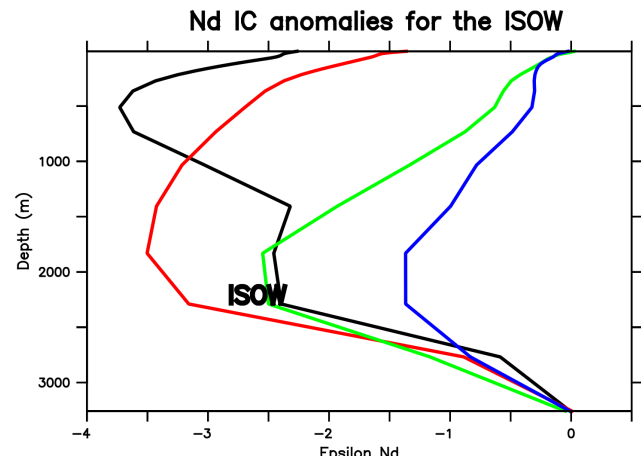
Figure 8. Comparison of Nd isotopic signature anomalies associated with the Iceland-Scotland Overflow Water (ISOW, at 56 °N 25 °W) identified between 2000 and 2600 m depth south of Iceland (Harvey and Theodorou, 1986) and the North Eastern Atlantic Deep Water (NEADW, at 50 °N 25 °W) between 2000 and 3000 m (Van Aken and de Jong, 2012), in HosMed2 (in black), HosMed1 (in red), HosMed05 (in green), and HosMed02 (in blue).
