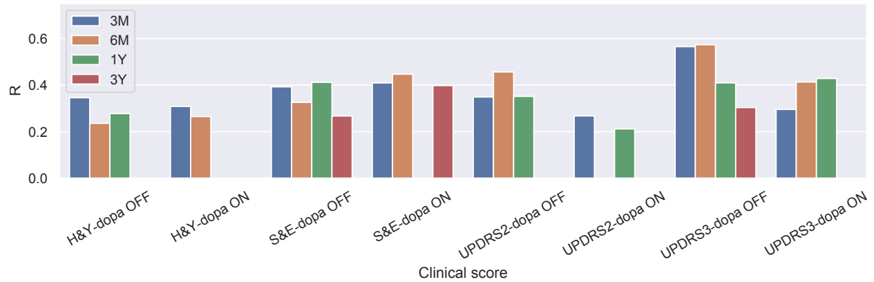
(a) Correlation coefficient of PassFlow predictions for motor tests.
