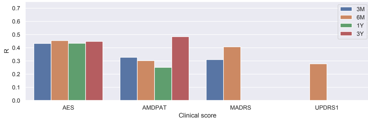
(b) Correlation coefficient of PassFlow predictions for behavioral tests.
