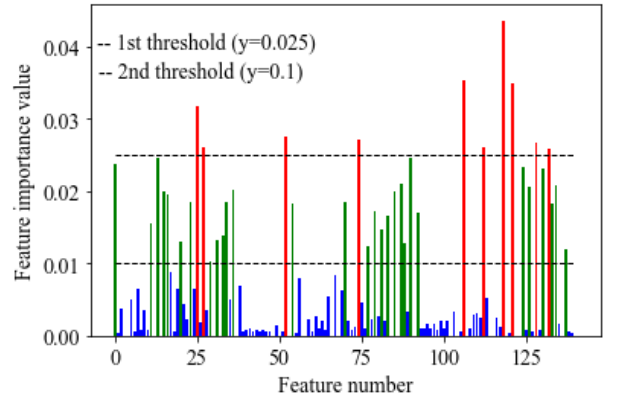
Fig. 6. Feature importance for the sensor placed in the pocket
