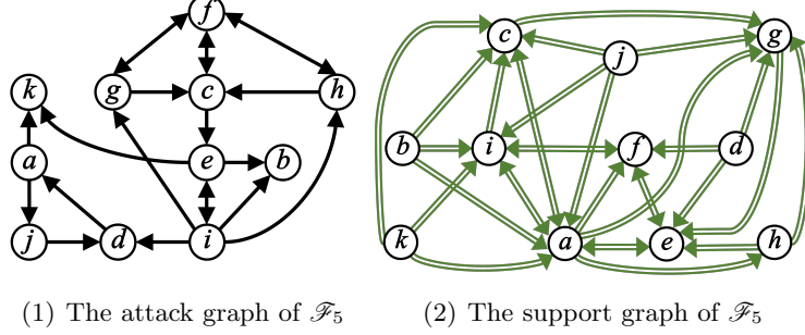
Figure 9: The BAF \mathcal{F}_5 .
