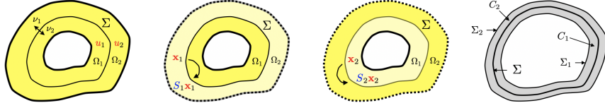
Fig. 1 The subdomains \Omega_1 and \Omega_2 (left). The scattering operators S_1 and S_2 (center). The layers C_1 and C_2 , cf section 5 (right)
