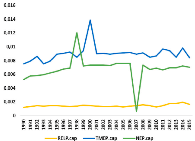
Fig. 3. Evolution of total electricity production, renewable electricity and nuclear electricity per capita (annual regional averages).
