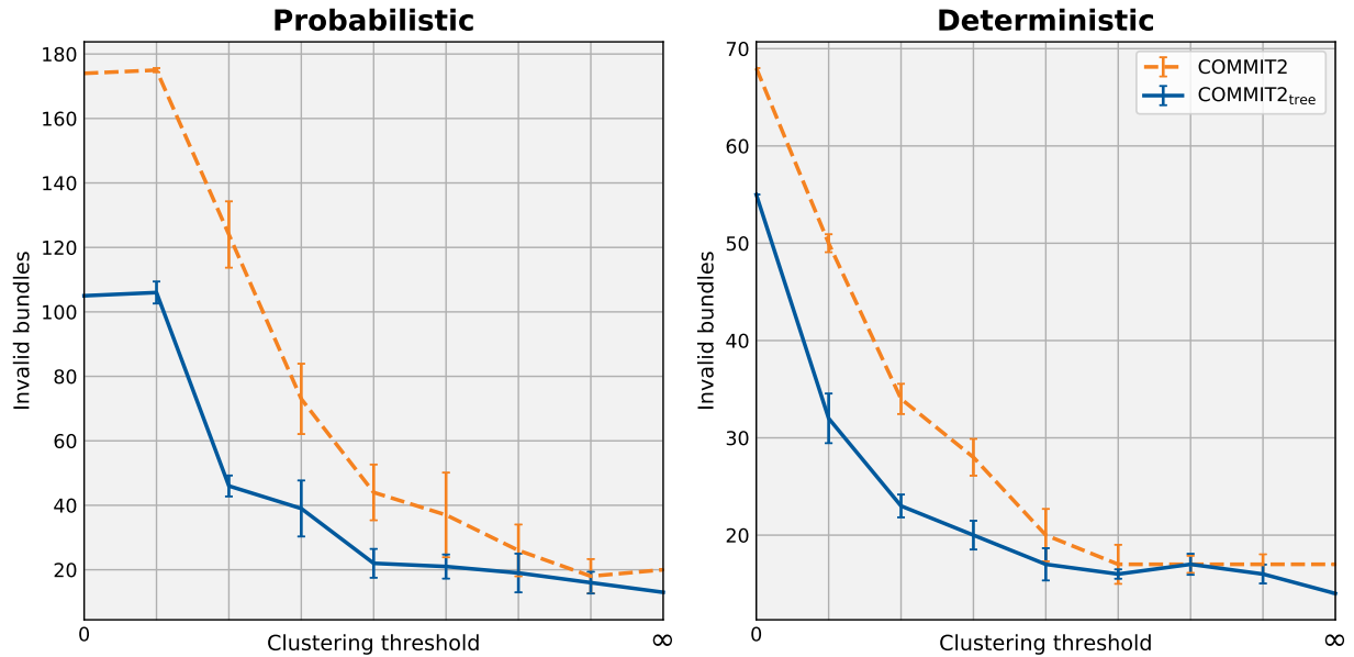
Supplementary Figure S2: Impact of the group size on the quality of the tractograms filtered with COMMIT2 tree . In the synthetic phantom, we investigated the effect of changing the size of the groups to build the second level of the hierarchy, by changing the threshold of the Average of Pointwise Euclidean Metric between streamlines from 0 (one streamline per cluster) to “infinity” (bundles are not clustered). We repeated the clustering 10 times and, here, we report the mean and standard deviation of invalid bundles kept after filtering with COMMIT2 tree (continuous blue line) and, for comparison, COMMIT2 (orange dashed line).
