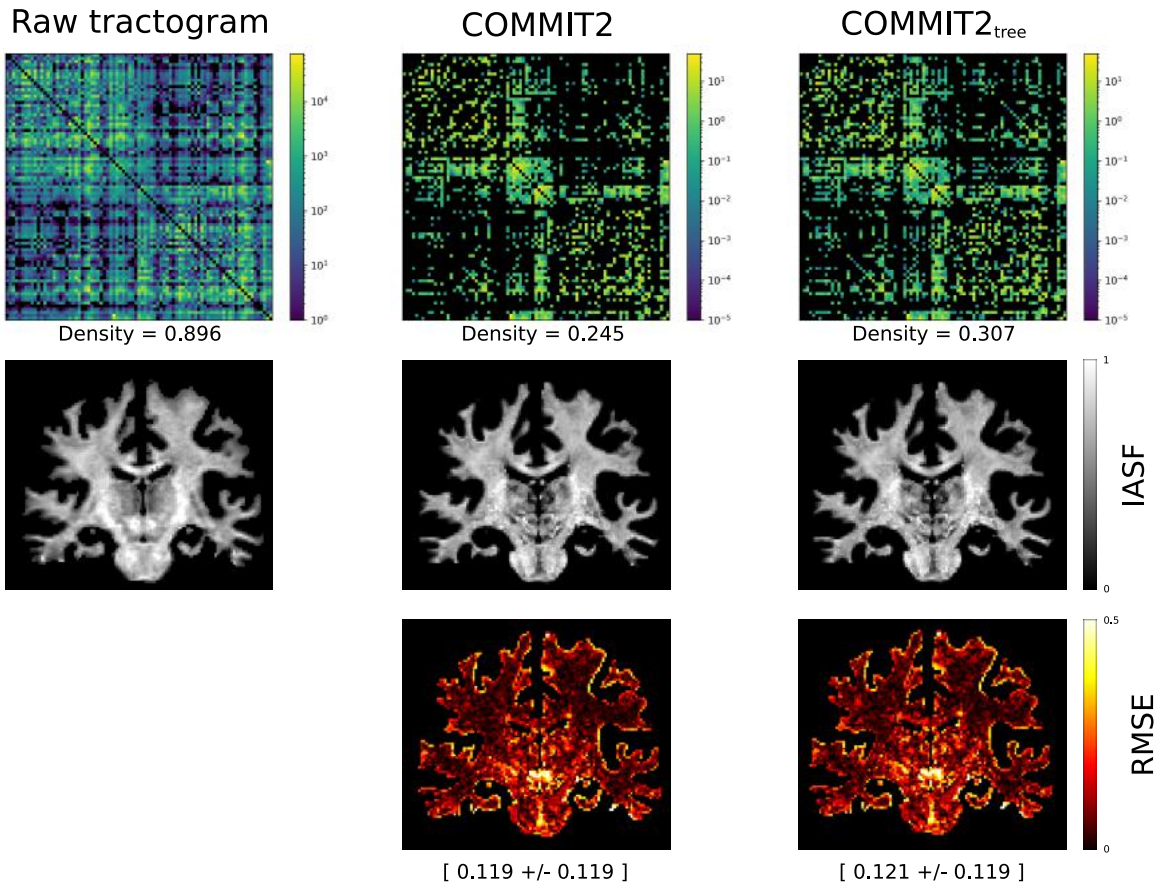
Figure 7: Connectomes estimated in one HCP subject. In the first row we show the estimated connectomes; in the case of the raw tractogram we used the number of streamlines, whereas for COMMIT2 and COMMIT2 tree the sum of the streamline contributions was used. In the second row we present the intra-axonal signal fraction (IASF) maps used as input and estimated to perform a visual inspection. The third row presents root mean square error (RMSE) maps of the estimations, along with their mean and standard deviation for a quantitative comparison.
