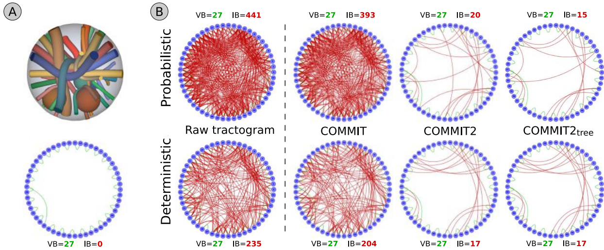
Figure 4: Quantitative comparison on synthetic data between COMMIT2 and COMMIT2 tree . We compared the valid (VB, reported in green) and invalid (IB, reported in red) bundles in the connectomes generated on a synthetic phantom (A, top) for which we know the ground-truth connectivity (A, bottom). Panel B compares the quality of the connectomes estimated from the probabilistic (top row) and deterministic (bottom row) tractograms before (raw tractogram) and after filtering with COMMIT2 and COMMIT2 tree ; performances of COMMIT are reported for reference.
