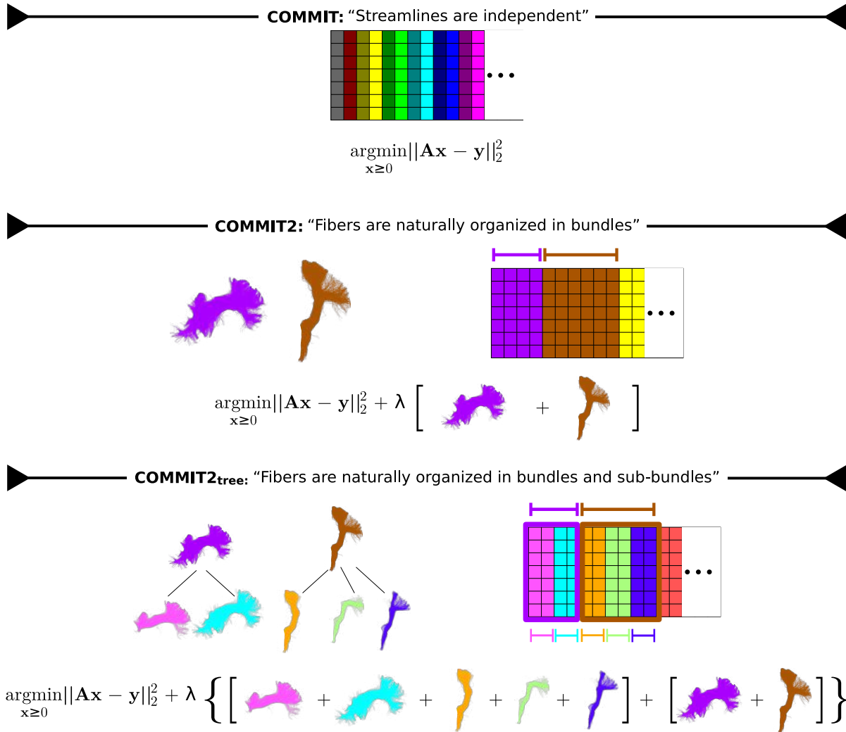
Figure 2: Visual comparison between the COMMIT, COMMIT2 and COMMIT2 tree formulations. COMMIT considered the streamlines as independent entities and COMMIT2 added a regularization term to take into account that streamlines are instead naturally organized in bundles. With COMMIT2 tree we propose to improve this regularization by allowing a multi-level hierarchical organization of the streamlines, where every bundle may be composed of several sub-bundles and each can be selectively promoted or penalized.
