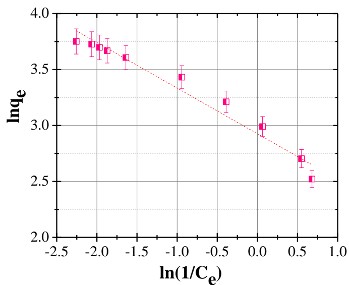
Figure 14. Harkin-Jura isotherm.
