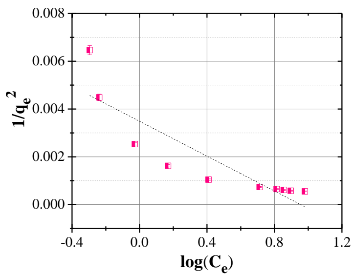
Figure 14. Harkin-Jura isotherm.
