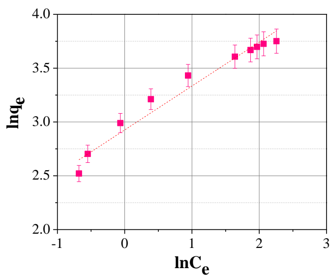
Figure 12. Freundlich isotherm.
