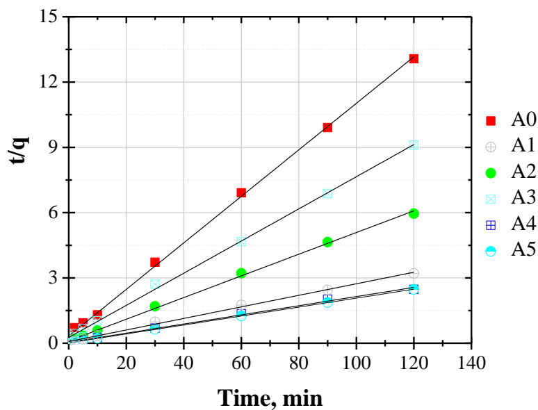
Figure 8. The fitting of the pseudo second-order model.
