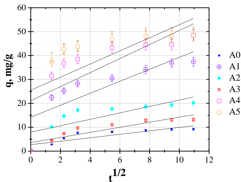
Figure 9. The fitting of the intraparticle diffusion model.
