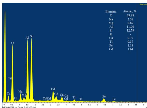
Figure 5b. SEM/EDS analysis after Cd(II) adsorption process
