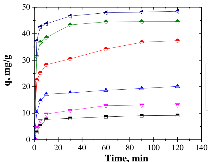
Figure 4. Influence of contact time and type of adsorbent on Cd (II) adsorption.
