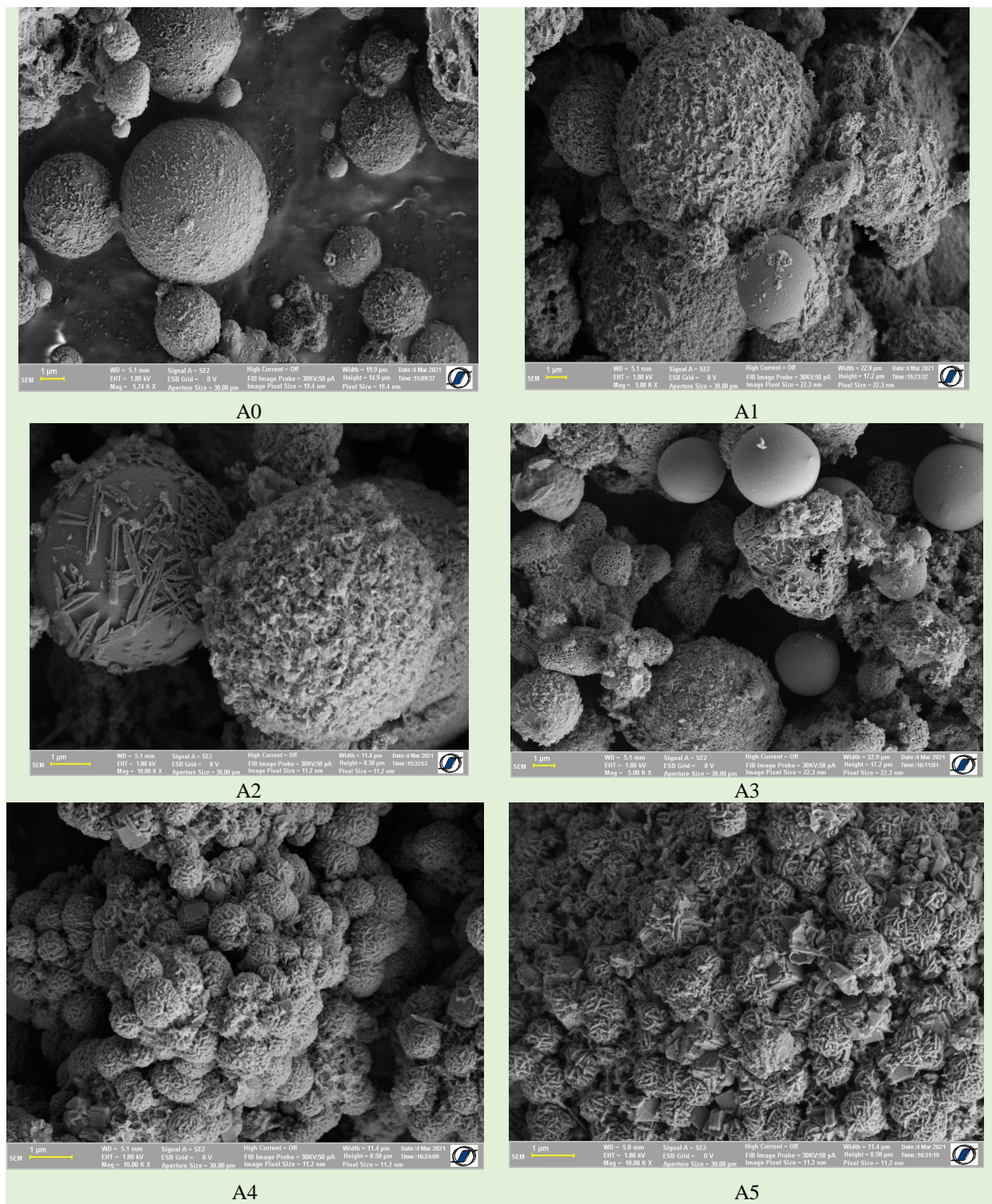
Figure 1. SEM images for A0 vs. A1–A5.
