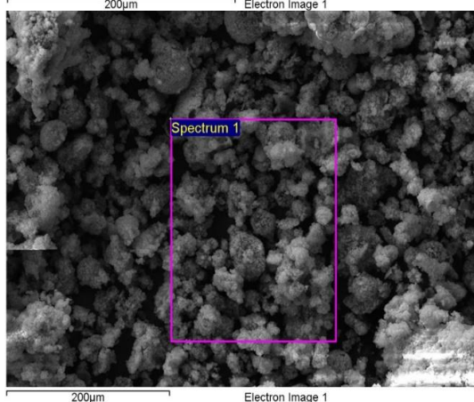
Figure 5b. SEM/EDS analysis after Cd(II) adsorption process
