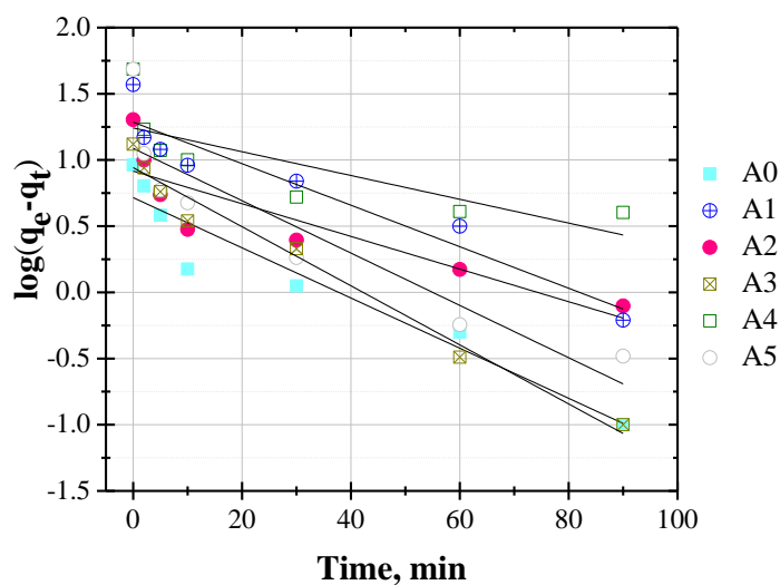
Figure 7. The fitting of the pseudo first-order model.
