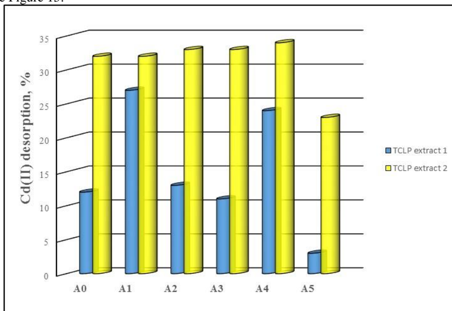
Figure 15. Desorption of Cd(II) from A0-A5 adsorbents
