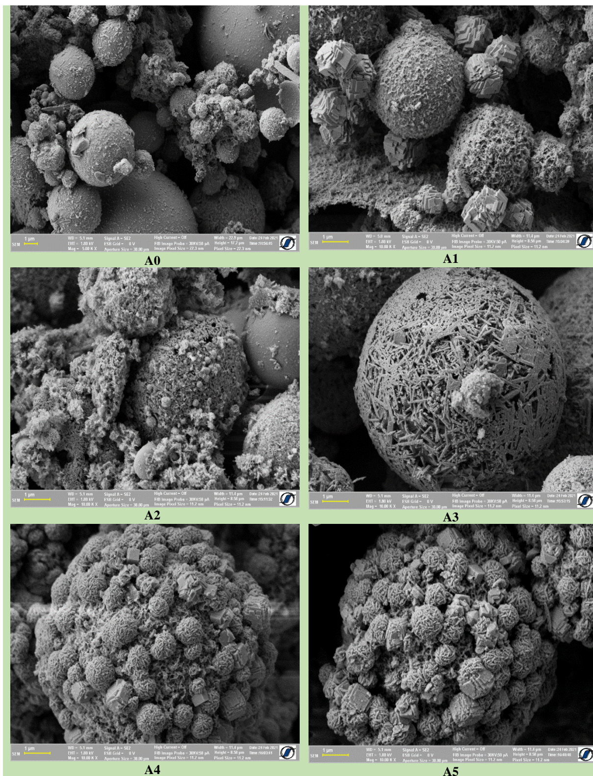
Figure 5a. SEM images of A0-A5 after Cd(II) adsorption process
