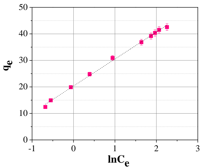
Figure 13. Temkin isotherm.
