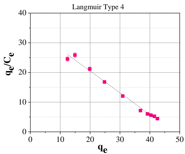
Figure 11. Langmuir isotherm.
