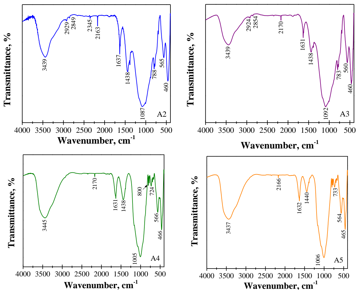
Figure 6. FTIR analysis after Cd(II) adsorption process
