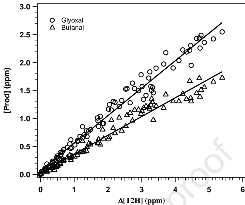
Figure 3. Plots of the concentrations of the glyoxal (O) and butanal ( \Delta ) as a function of reacted T2H (FTIR analysis) obtained in the 480-L chamber (without OH scavenger)
