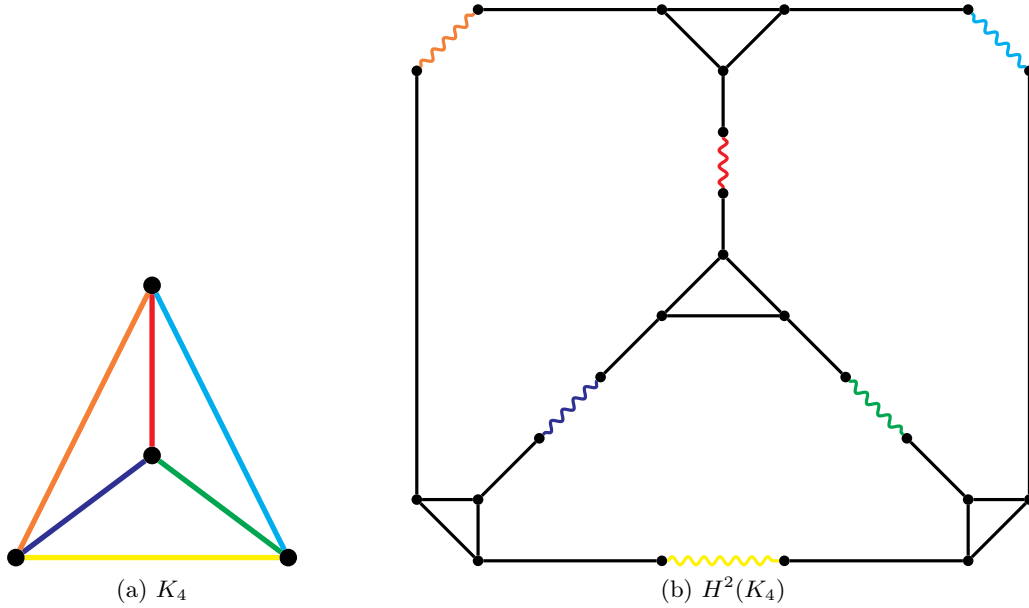
Figure 3: The construction described in Subsection 2.3, performed from r = 2 and the complete graph K_4 on four vertices. The colours indicate the equivalence between the edges of K_4 and some edges of H^2(K_4) .
