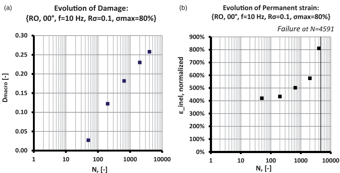
Figure 21. Evolution of (a) damage and (b) permanent strain, for a RO-00 ° sample loaded under ( f=10 Hz, R\sigma=0.1 , \sigma_{max}=80\% ). RO: randomly oriented.
