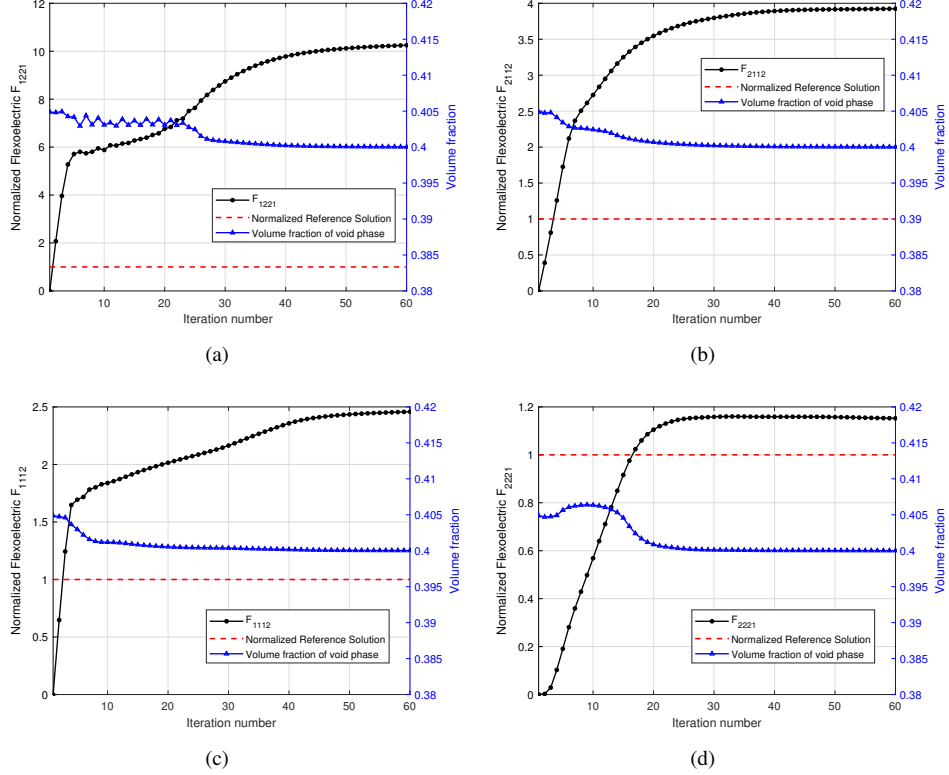
Figure 16: Topology optimization process with respect to normalized flexoelectric components and volume fractions for the PZT/void: (a) \bar{F}_{1221} ; (b) \bar{F}_{2112} ; (c) \bar{F}_{1112} ; (d) \bar{F}_{2221} .
