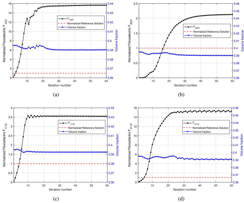
Figure 12: Topology optimization process with respect to normalized flexoelectric components and volume fractions for the PVDF/PZT: (a) \bar{F}_{1221} ; (b) \bar{F}_{2221} ; (c) \bar{F}_{1112} ; (d) \bar{F}_{2112} .
