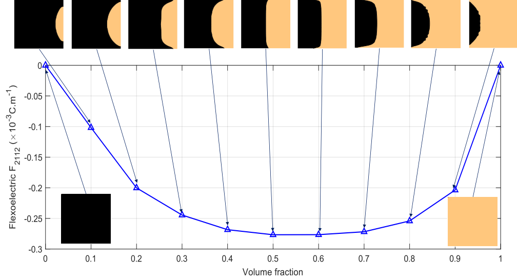
Figure 9: Optimal values of flexoelectric coefficient \bar{F}_{2112} and corresponding topologies with respect to volume fraction of inclusion.
