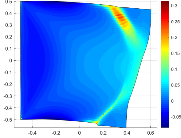
Figure 14: Deformation and strain \epsilon_{22} of optimized unit cell in Fig. 7c induced by electric field E_2
