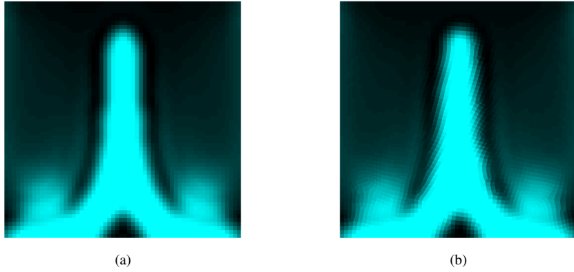
Figure 13: Optimal topology for \bar{F}_{2221} on PZT/polymer: (a) with regular meshing; (b) with irregular meshing
