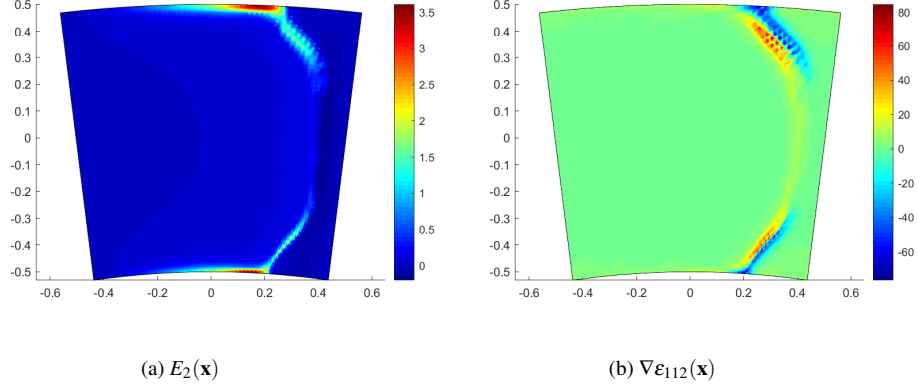
Figure 15: Electric field ( E_2 -component) and strain gradient ( \nabla\epsilon_{112} -component) within the PZT-PVDF-optimized microstructure shown in Fig. 7(c).
