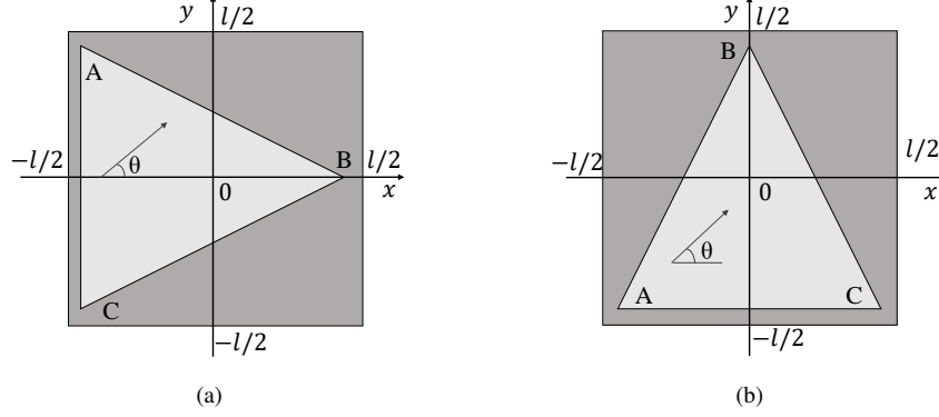
Figure 2: Unit cells with triangular inclusions with inclusion volume fraction of f = 0.4 , polarization P and the mismatch angle \theta between matrix and inclusion phases; (a) guess design used for computing \bar{F}_{1221} and \bar{F}_{2112} ; (b) guess design used for computing \bar{F}_{1112} and \bar{F}_{2221} .
