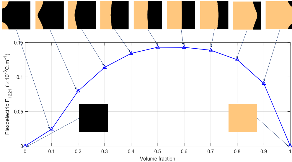
Figure 8: Optimal values of flexoelectric coefficient \bar{F}_{1221} and corresponding topologies with respect to volume fraction of inclusion.
