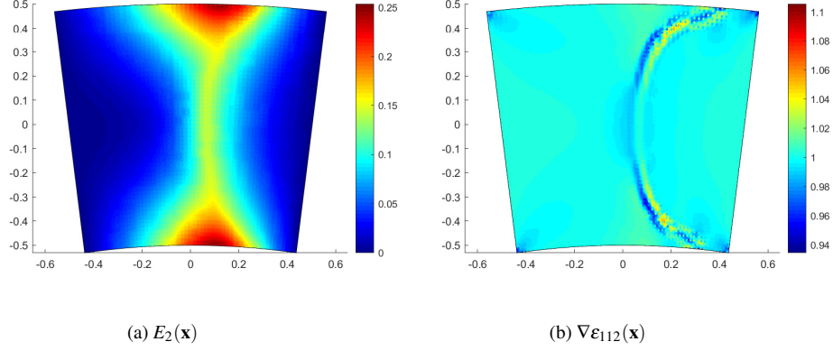
Figure 5: Electric field ( E_2 -component) and strain gradient ( \nabla \varepsilon_{112} -component within the PZT-PZT-optimized microstructure corresponding to the optimized \bar{F}_{2112} in Fig. 7(a).
