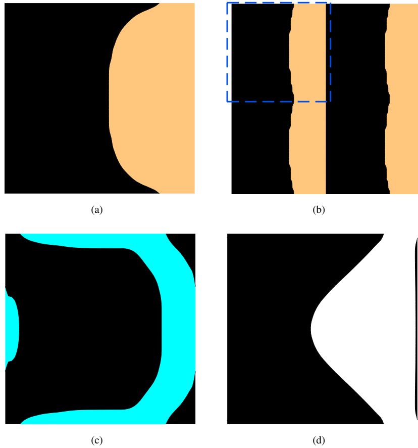
Figure 7: Optimal topology for \bar{F}_{2112} : (a) PZT/PZT, 1 \times 1 cells; (b) PZT/PZT, 2 \times 2 cells; (c) PZT/polymer, 1 \times 1 cells; (d) PZT/void, 1 \times 1 cells.
