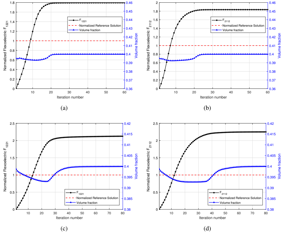
Figure 3: Topology optimization process with respect to normalized flexoelectric components and volume fractions for the PZT/PZT: (a) \bar{F}_{1221} , 1 \times 1 cells; (b) \bar{F}_{2112} , 1 \times 1 cells; (c) \bar{F}_{1221} , 2 \times 2 cells; (d) \bar{F}_{2112} , 2 \times 2 cells.
