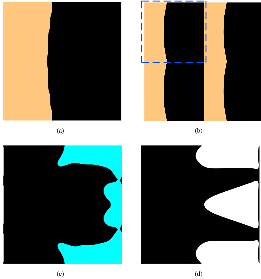
Figure 4: Optimal topology for \bar{F}_{1221} : (a) PZT/PZT, 1 \times 1 cells; (b) PZT/PZT, 2 \times 2 cells; (c) PZT/polymer, 1 \times 1 cells; (d) PZT/void, 1 \times 1 cells.
