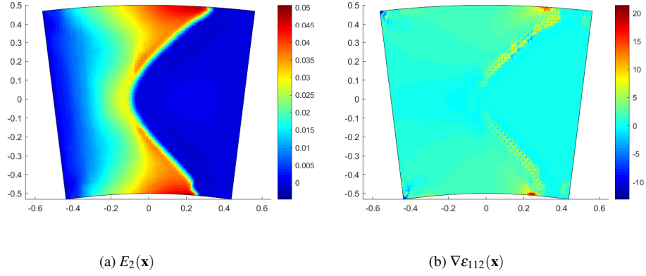
Figure 17: Electric field ( E_2 -component) and strain gradient ( \nabla\epsilon_{112} )-component within the PZT-void-optimized microstructure in Fig. 7(d).
