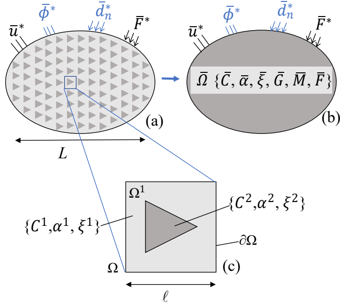
Figure 1: (a) Periodic heterogeneous structure; (b) Equivalent piezo-flexoelectric homogeneous structure; (c) RVE model
