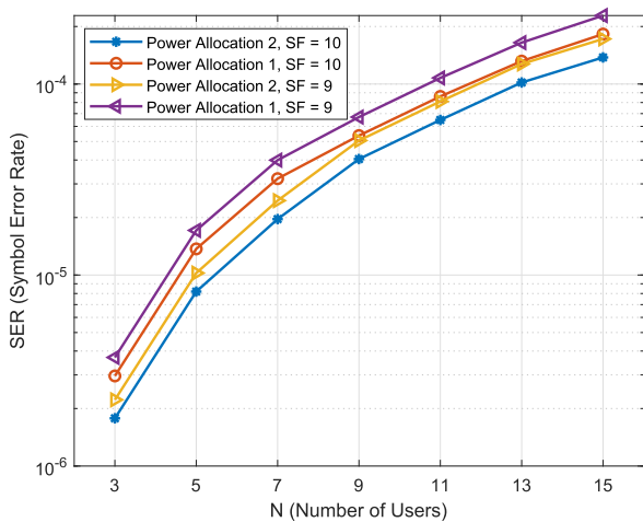
FIGURE 9. SER of the proposed MUD for different N , Noise level of -114 dBm, SF = 9, 10, and B = 250 kHz.
