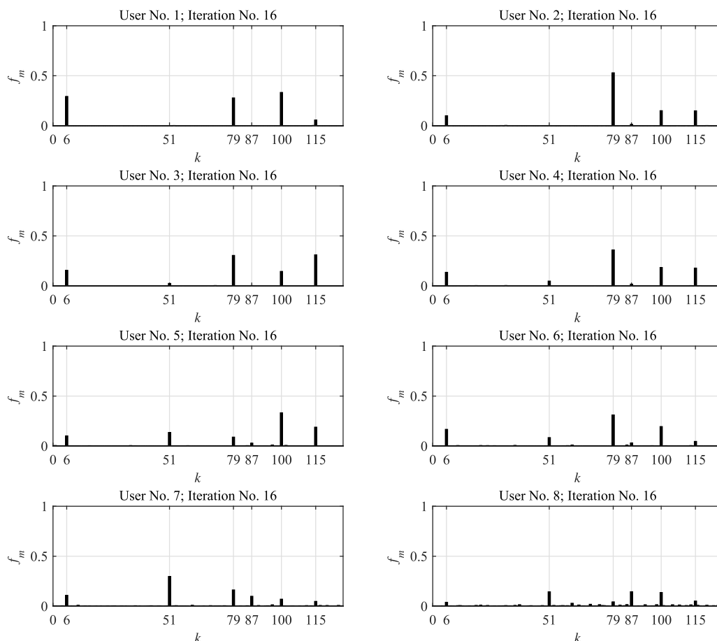
FIGURE 3. CEM-MUD as per Algorithm 1, with N = 8 users and SF = 7. In this example two collisions occur ( \mathbf{m}_q = \{6, 79, 115, 79, 100, 100, 51, 87\} ). The figures represent f_m at the beginning of the 16th iteration. We can see that if values tend to gain in probability, the decision cannot be made yet.
