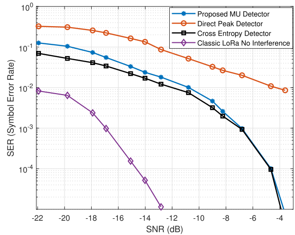
(b) Performance of a single user in the presence of 9 interfering users.
