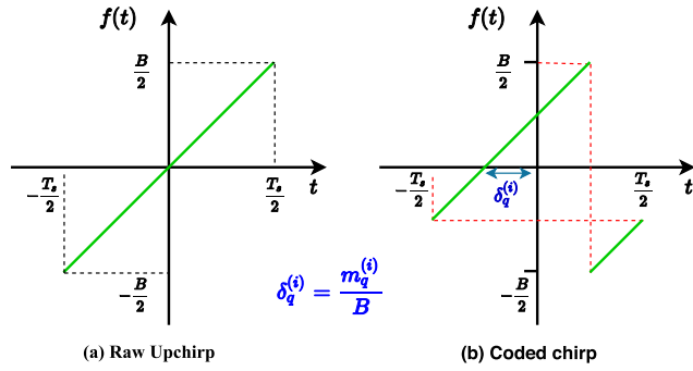
FIGURE 1. Raw chirp and Coded chirp associated with m_q^{(i)} .
