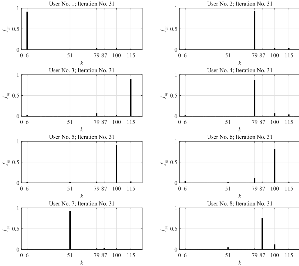
FIGURE 4. CEM-MUD as per Algorithm 1, with N = 8 users and SF = 7 . In this example two collisions occur ( \mathbf{m}_q = \{6, 79, 115, 79, 100, 100, 51, 87\} ). The figures represent f_m at the beginning of the 31st iteration. We can see that for each user the probability is clearly converging towards a single value equal to one, all the others being zero. We also see that the decision is good despite the two collisions that occur between users 2 and 4 and users 5 and 6.
