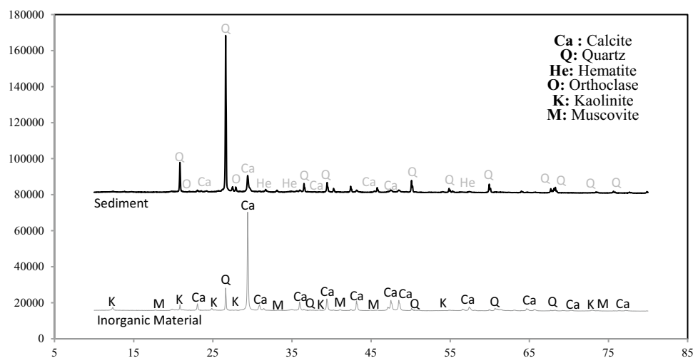
Fig. 2 XRD spectra of sediment and inorganic material
