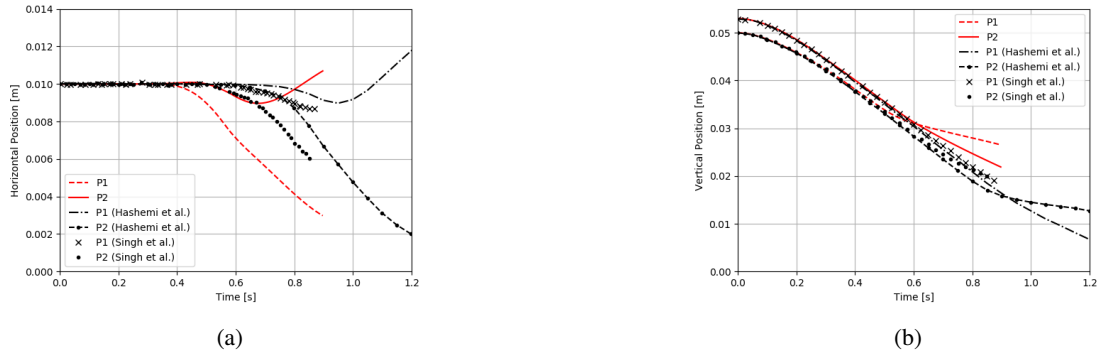
Figure 12: Position of the solid particles for the (a) x-position and (b) y-position
