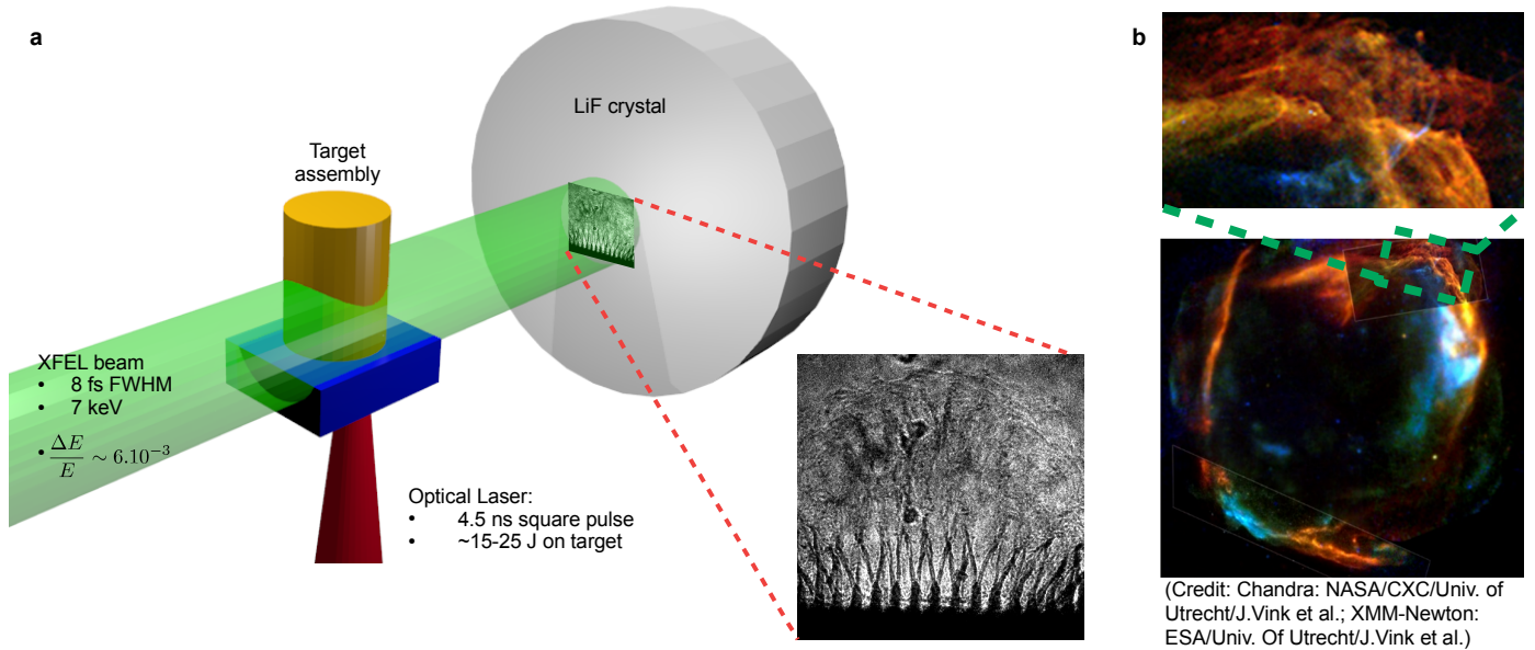
FIG. 1. Experimental setup. Diagram of the overall experiment setup (a) and Chandra's observation of RCW 86 (b). The plasma expansion inside the laser driven target is diagnosed using a XFEL beam ( >1 mm diameter, 8 fs, centred on a 7 keV emission with a \Delta E/E = 6 \times 10^{-3} ) and lithium fluoride crystal. This expansion is Rayleigh-Taylor unstable, as in the supernovae remnant.
