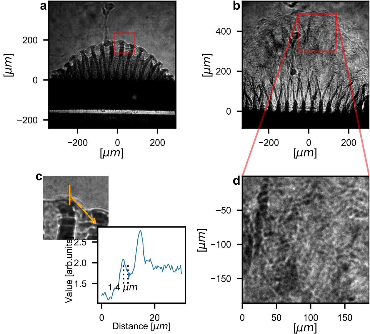
FIG. 2. Experimental radiographs of the mono-mode targets. Experimental radiographs of mono-mode targets obtained before (40 ns (a) and (c)) and after (60 ns (b) and (d)) the transition to turbulence between 50 ns and 60 ns. Following the initial Rayleigh-Taylor growth and pusher expansion (curved modulated surface of the two first radiograph), the system becomes turbulent. The structure becomes blurry and the power spectrum nearly isotropic, as can be observed on the zoom of the 60 ns radiograph. A precise study was made possible thanks to the high resolution of the radiography, which is illustrated on the zoom and line-out of the 40 ns radiograph (c).
