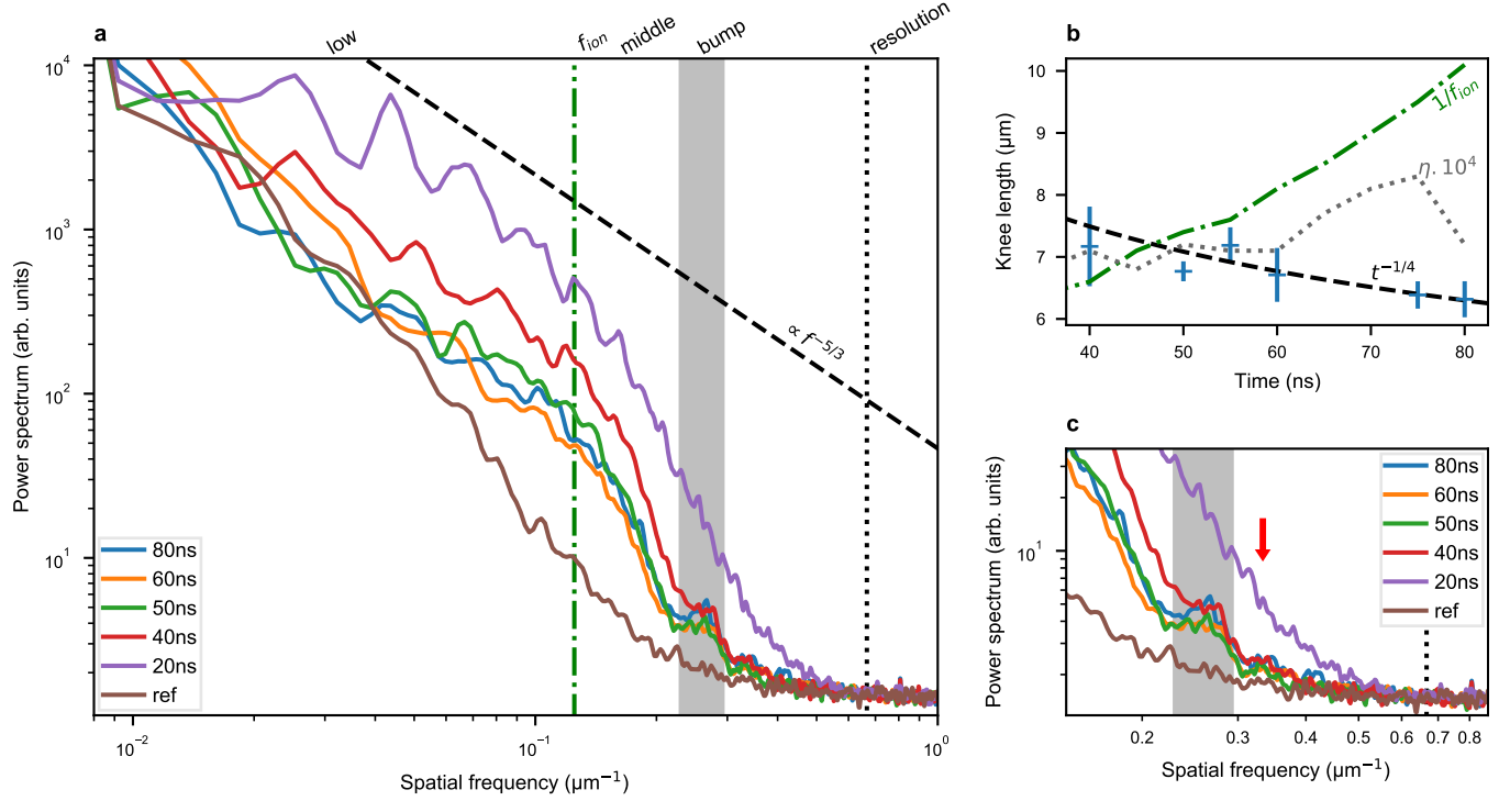
FIG. 4. Spatial power spectra of the turbulent zone. Spatial power spectrum (a), temporal evolution of the knee position (b) and bump morphology (c). a) Typical radial power spectrum of the turbulent plasma obtained, at different times after the laser drive, compared to a reference case, non-shocked foam. The “low” spectrum evolved as a power law consistent with turbulence theory: a fiducial with a -5/3 coefficient is marked by dashes. The middle zone follows a power law with a much higher coefficient (nearly -6.6 in the 60 ns spectrum). The spatial frequency corresponding to the ion inertial range at 50 ns, f_i , is marked by the dash-dot line and is near the inflexion of the spectrum. The bump is highlighted by the grey zone, and is abnormal considering classical turbulence theory. The nearly flat spectrum, for spatial frequency above the bump, corresponds to the resolution limit of our diagnostic. b) Evolution of the knee position as a function of time. The data points correspond to the mean values of our data set with a standard deviation as error bars. The dashed fiducial corresponds to a t^{-1/4} evolution. The dotted line corresponds to the simulated Kolmogorov scale (as calculated in table II for the hydrodynamic mono-mode case) time of 10^4 . The green dash-dotted line to the theoretical ion inertial range. c) Comparison of the bump morphology at different times. The greyed zone highlights the bump position. The red arrow marks the phase contrast wavelength measured on grids.
