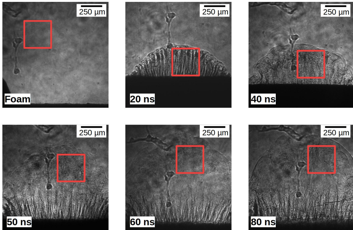
FIG. 3. Experimental radiograph showing the dynamic of the bi-mode targets. The position of the ROI taken to calculate the spectrum of figure 4 are shown with a red square.
