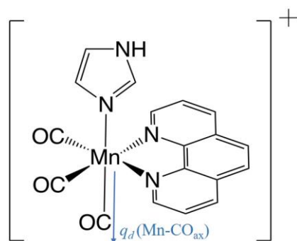
Scheme 1. Structure of [\text{Mn}(\text{im})(\text{CO})_3(\text{phen})]^+ together with the axial CO release mode, q_d ( \text{Mn-CO}_{\text{ax}} ).
