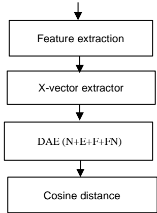
Figure 2. General domain adaptation for different distortions
