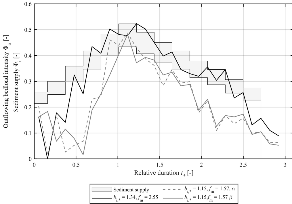
Fig. 10. Hybrid barrier: Outflowing bedload intensity, \Phi_o , and the sediment supply intensity, \Phi_i , as a function of the relative hydrograph duration, t_* , for the combined mechanical hydraulic deposition control. The plot shows the optimal design with a relative bar spacing of b_{i,*} = 1.15 and a relative bottom clearance height of f_m = 1.57 compared to a bar screen with b_{i,*} = 1.34 and f_m = 2.55 originally designed for coarser sediment. A very fast increase of \Phi_o indicates self-flushing and \Phi_o \geq \Phi_i indicates a barrier that is literally transparent for sediment transport.
