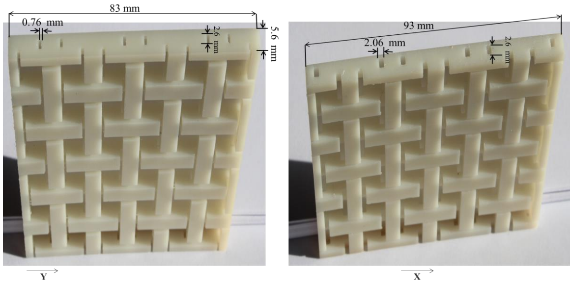
Fig. 8: The side view of the porous medium in assumed X and Y directions: the dimensions of two pore structures (left) the rectangular channels with identical widths of 0.76 mm, (right) the rectangular channels with identical widths of 2.06 mm
