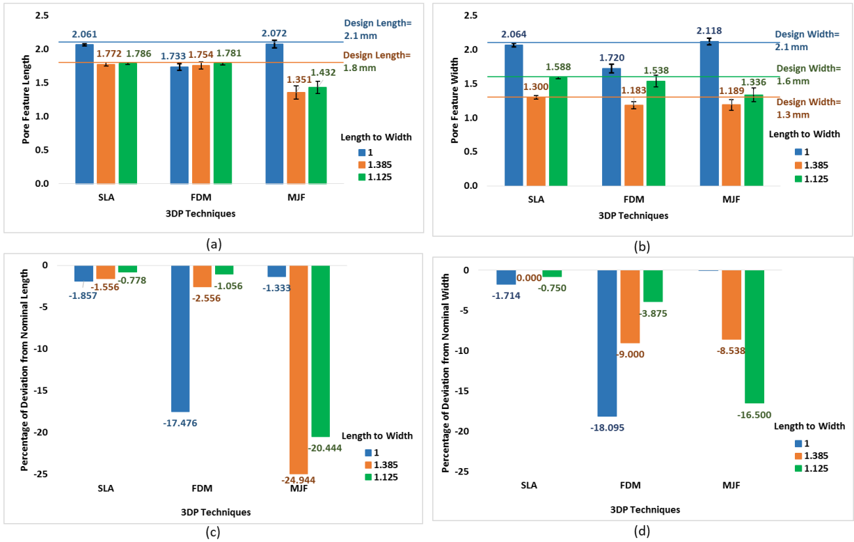
Fig. 7: Average measured length (a) and width (b) and percentage of deviation from nominal (c) length and (d) width of pore features with different design ratio of length to width fabricated by different 3DP techniques
