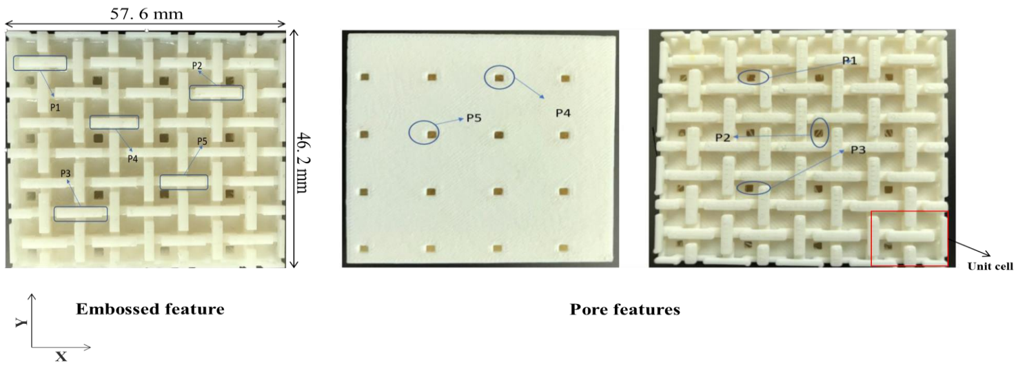
Fig. 4: Photographs indicating dimensions of the textile-like porous medium: five random locations used for measurement of the selected features.
