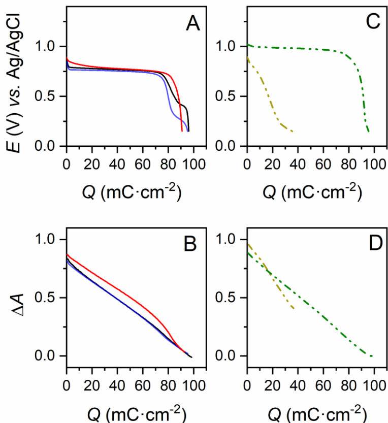
Figure 1. In operando spectroelectrochemical characterization of the first discharge of MnO 2 -GLAD-ITO electrodes in different aqueous electrolytes (all adjusted to pH 2.0 except for dashed olive data corresponding to pH 1.0). (A, C) Galvanostatic curves (rate: 0.3 mA·cm -2 ) and (B, D) absorbance variations concomitantly recorded at MnO 2 -GLAD-ITO electrodes (loaded ex situ with a deposited charge of 100 mC·cm -2 ) immersed in the following electrolytes: (red) 1 M acetic acid + 0.1 M MnCl 2 + 2 M KCl, (blue) 1 M Al(OTf) 3 + 0.1 M MnCl 2 , (plain black) 1 M AlCl 3 + 0.1 M MnCl 2 , (dashed lines) 2 M KCl + 0.1 M MnCl 2 adjusted to (dark yellow) pH 2.0 or (olive) pH 1.0.
