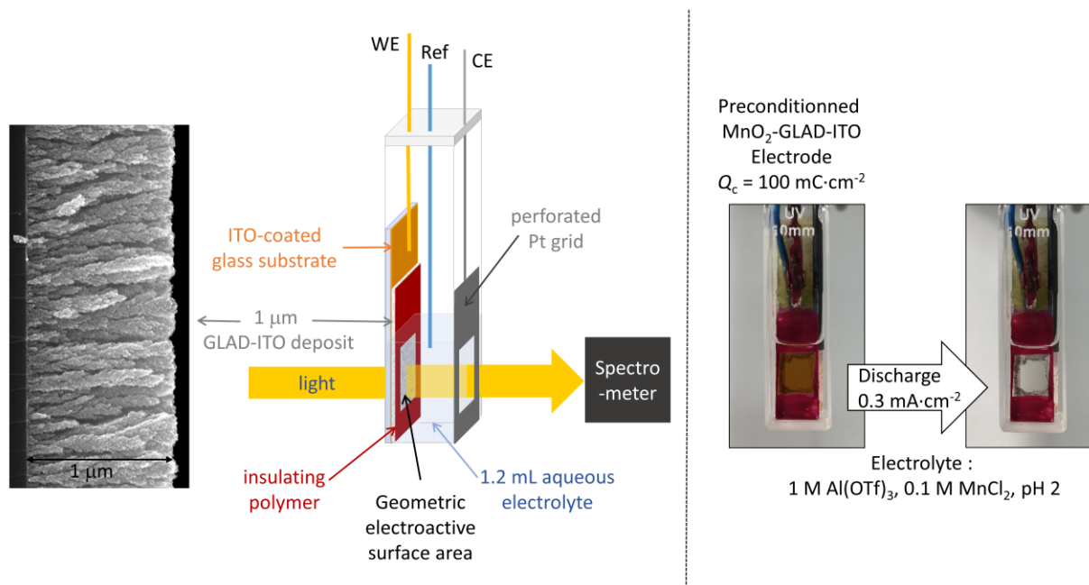
Scheme 1. Left: schematic of the in operando spectroelectrochemical setup used to monitor a \text{MnO}_2 -loaded GLAD-ITO electrode (made of a 1\text{-}\mu\text{m} thick transparent nanostructured film of GLAD-ITO). Right: photographs of the spectroelectrochemical cell taken at the beginning and end of a galvanostatic discharge experiment performed at a GLAD-ITO electrode loaded ex situ .
