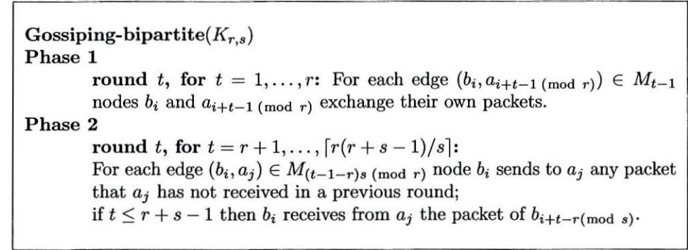
FIG. 6. Gossiping algorithm in K_{r,s} .
