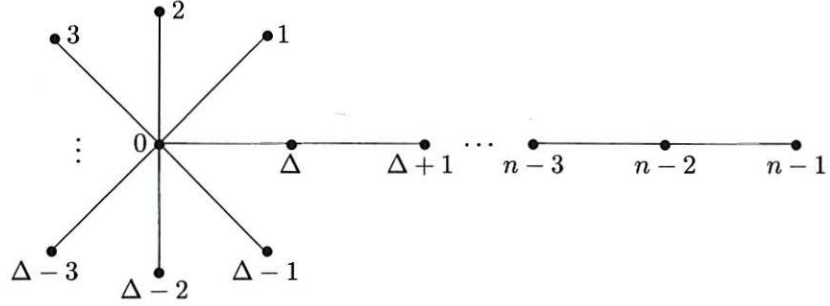
FIG. 4. Tree S_{n, \Delta} .
