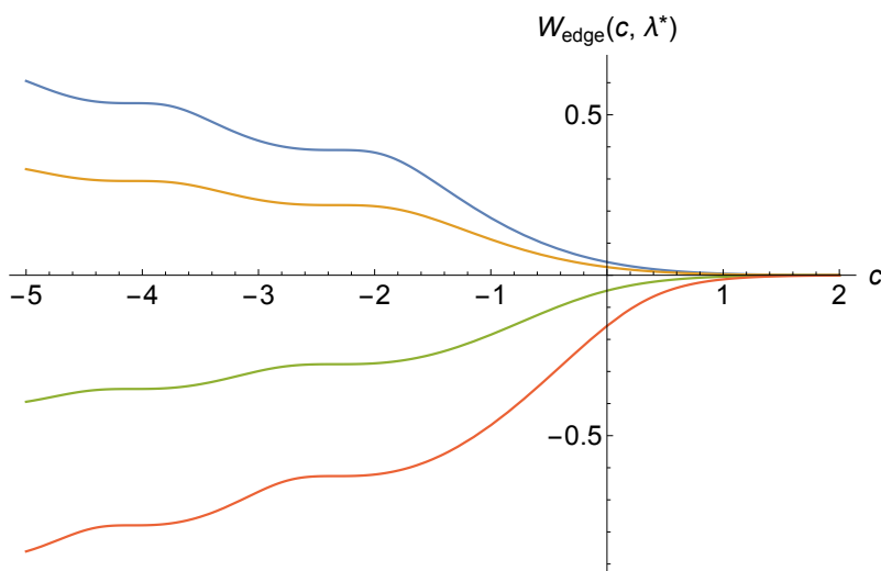
Figure 8: The scaled potential W_{\text{edge}}(c, \lambda^*) felt by an impurity at the edge as a function of the distance c from the edge measured in units of w_e as given in Eq. (135). Shown from top to bottom is the potential for \lambda^* = 1, 0.5, -0.5, -1 .
