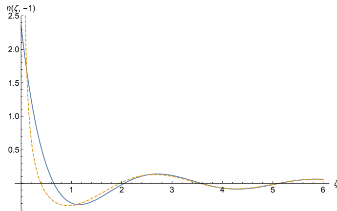
Figure 5: The relative change in the density around the point x = x_1 , given by Eq. (71) due to an attractive delta function potential at the point x = 0 of amplitude such that \lambda = -\lambda_A = \gamma k_F for \gamma = -1 (solid line), and its asymptotic approximation (dashed line) using Eq. (69).
