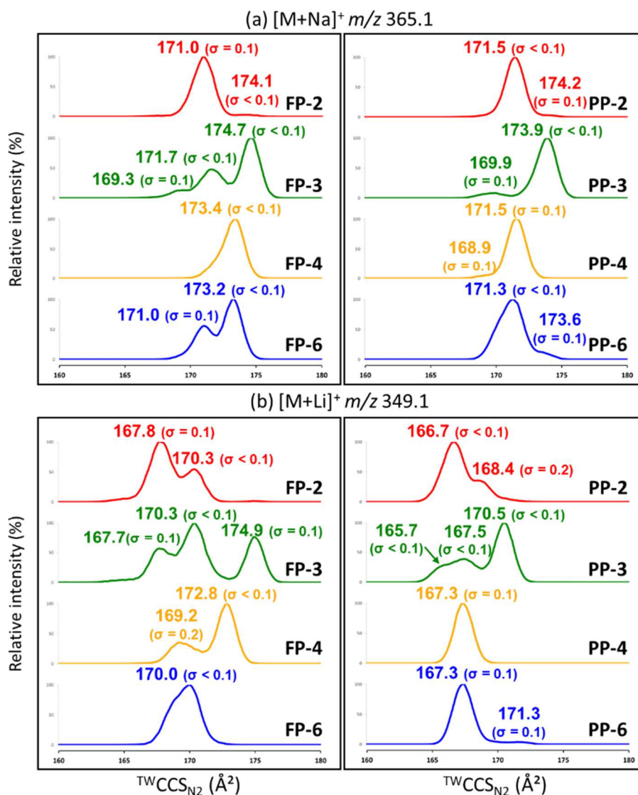
Figure 2. Extracted monoisotopic ion mobility spectra for the eight synthesized products as (a) [M+Na]^+ ( m/z 365.1) and (b) as [M+Li]^+ ( m/z 349.1). Standard deviations are given for three replicates. For both parts, left panel corresponds to the galactofuranosyl containing disaccharides and right panel to the pyranosyl-containing ones. Color for the regiochemistry of the glycosidic bond: Gal-(1→2)-Man (red), Gal-(1→3)-Man (green), Gal-(1→4)-Man (orange), and Gal-(1→6)-Man (blue).
