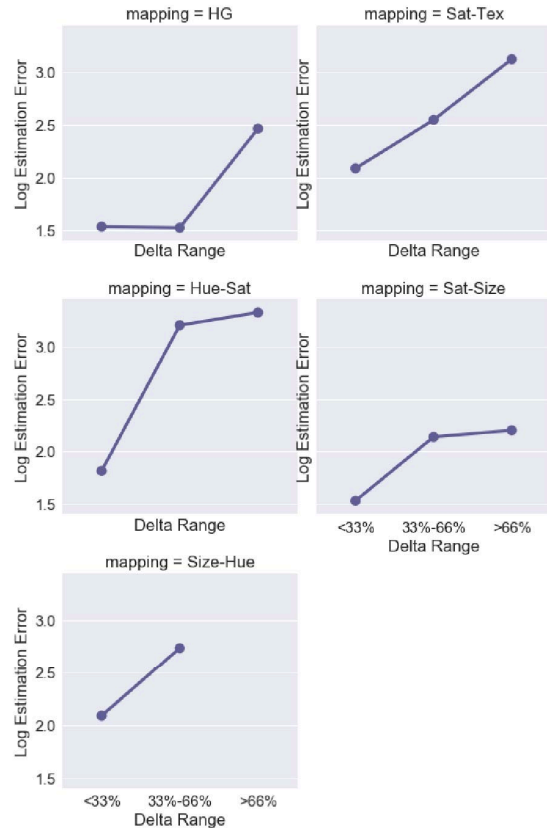
Figure 12: Effect of the real value difference on logarithmic error: comparing the five mappings.
