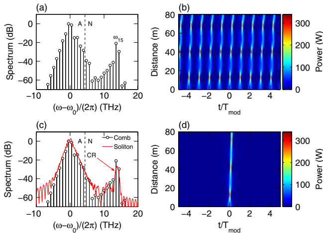
FIG. 2 (color online). Simulation showing amplification at \omega_{15} in (a) frequency and (b) time domains. To establish the link with soliton-induced Cherenkov radiation, (c) compares the discrete comb spectrum with that of a soliton pulse corresponding to one cycle of the initial modulation. (d) Time-domain evolution. The mean pump frequency is \omega_0/2\pi = 188.5 THz and the pump detuning is \Delta/2\pi = 0.87 THz.
