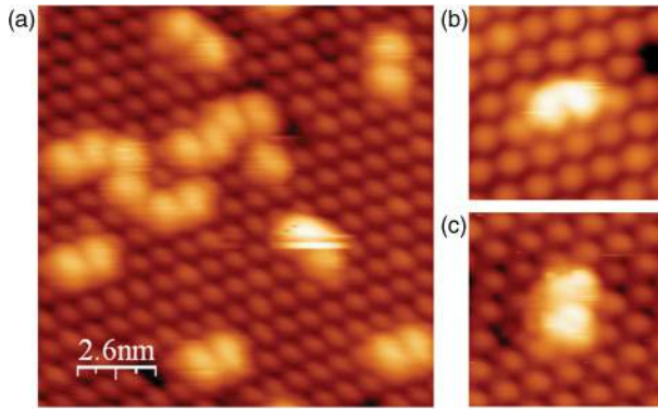
FIG. 1. (Color online) (a) STM image of DHH-PTCDI molecules adsorbed on the SiC(0001)- 3 \times 3 surface (image size 21 \times 21 nm; tunneling conditions -2.0 V and 0.3 nA). [(b),(c)] Images showing close-ups of two single molecules and their position with respect to the surface adatoms (image size 5 \times 5 nm; tunneling conditions -3.0 V and 0.3 nA).
