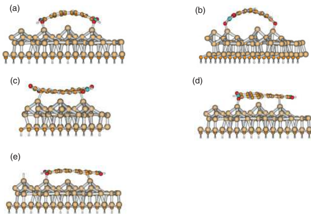
FIG. 4. (Color online) Side views of the optimized configurations of the five models investigated in this work: (a) M1, (b) M2, (c) M3, (d) M4, and (e) M5. The colors used to designate the atoms are the same as in Figs. 2 and 3.
