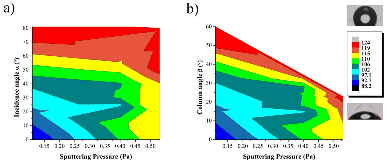
Figure 16: Pseudo 3D-maps displaying the evolution of the average contact angle \theta of a water drop (in °) as a function of the sputtering argon pressure and (a) the incidence angle \alpha and (b) the column angle \beta
