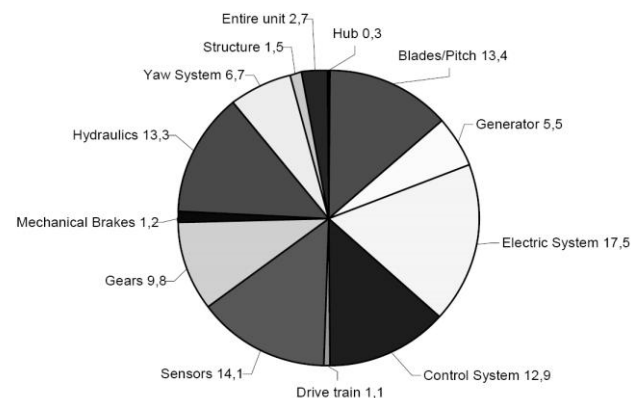
(a) Failures number distribution for Swedish wind power plants (2000-2004).
