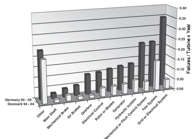
(b) Failure rates for Danish and German wind power plants.
