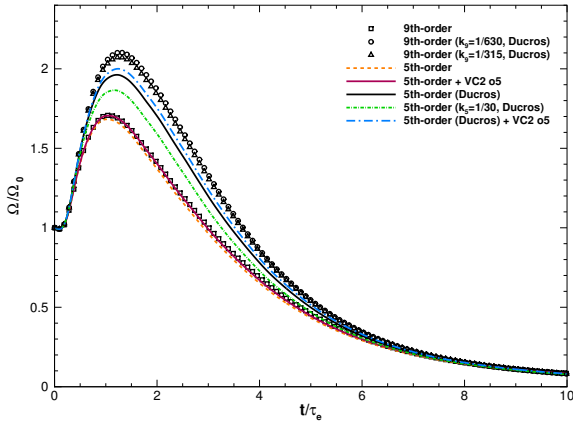
Figure 2: Time evolution of enstrophy at M_{T0} = 1.0 for different numerical schemes.
