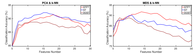
Figure 7: Classification accuracy by features number
