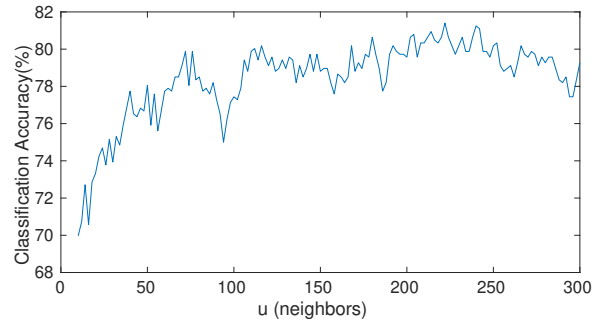
Figure 6: Isomap - Classification accuracy by number of neighbours in Isomap algorithm
