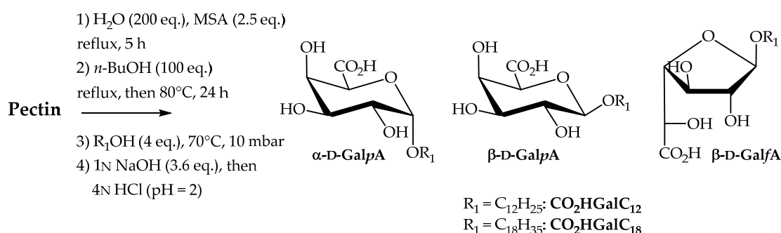
Scheme 4. Transformation of pectin into n -alkyl D-galactosiduronic acids \text{CO}_2\text{HGalC}_n .
