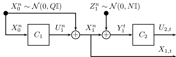
Fig. 1. The state and the channel noise are drawn according to the i.i.d. Gaussian distributions X_0^n \sim \mathcal{N}(0, Q\mathbb{I}) and Z_1^n \sim \mathcal{N}(0, N\mathbb{I}) . The interim state sequence X_1^n is causally estimated by decision maker C_2 .
