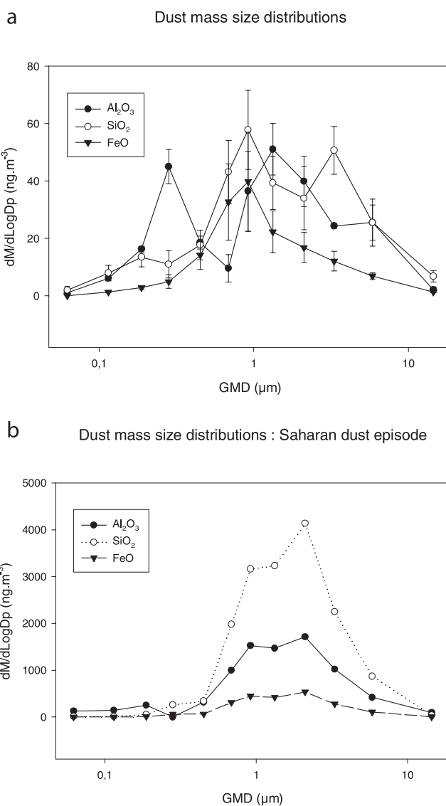
Figure 6. Dust mass size distributions for (a) all analyzed samples but sample 11 and (b) sample 11 (Saharan dust episode).
