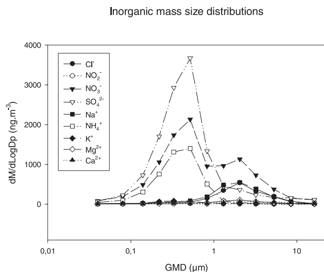
Figure 5. Mass distribution for inorganic ions for all analyzed samples.
