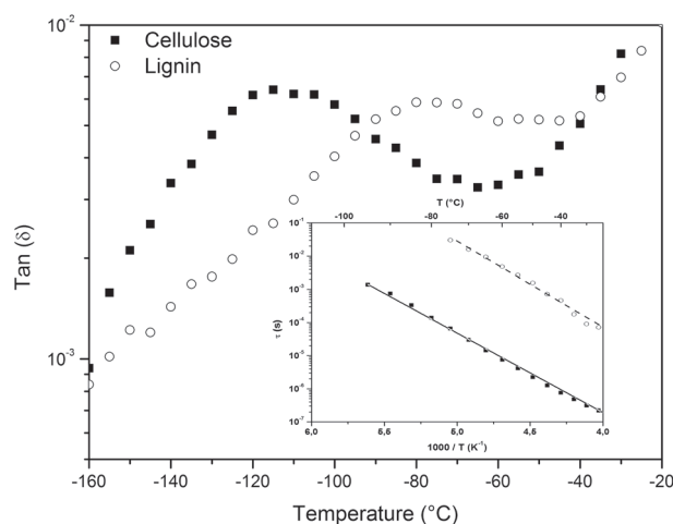
Fig. 1 Dielectric \tan\delta versus temperature at the frequency F = 1 Hz of the low-temperature relaxation mode observed by DDS for cellulose (black square) and lignin (open circle); inset Arrhenius diagram of the average relaxation time from 10^{-1} to 10^{+6} isofrequencies
