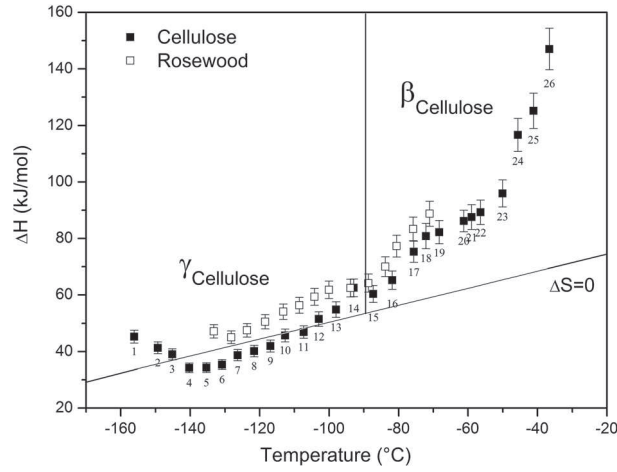
Fig. 7 Activation enthalpy of the elementary TSC thermograms as a function of temperature for cellulose (black square) and rosewood (open square). The Starkweather line \Delta S = 0 is indicated as reference
