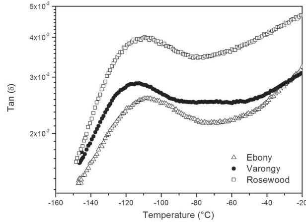
Fig. 8 Mechanical \tan \delta versus temperature at the frequency F = 1 Hz for the low-temperature relaxation mode observed by DMA for varongy (filled circle), rosewood (open square) and ebony ( \Delta )
