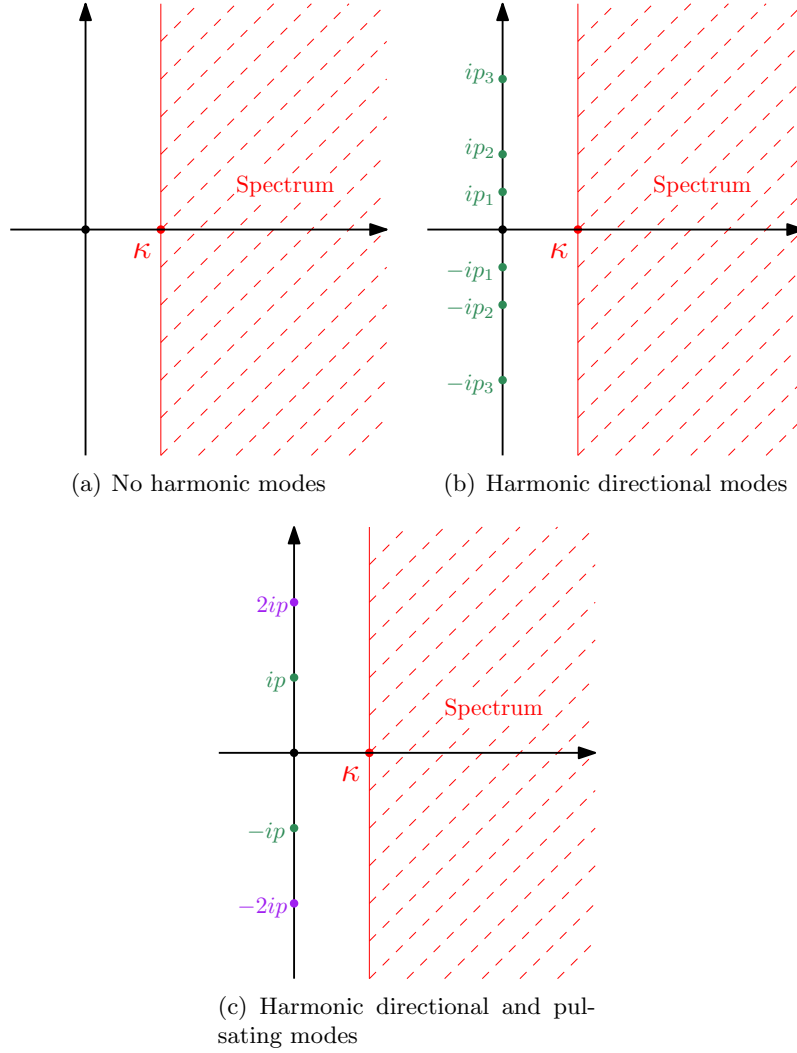
FIGURE 1. Complex spectrum of -\mathcal{L} .
