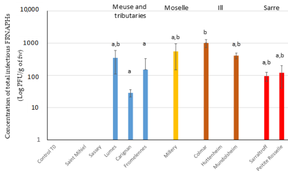
Figure 2. Concentrations of total infectious F-specific RNA bacteriophages (FNRAPHS) (mean \pm SD, N = 3; PFU/g fw) quantified in the fresh weight (fw) of zebra mussel soft tissue before (control, T0) and after their introduction at the different sites for two months. Histograms marked with the same letter (a,b) are not statistically different at the 95% significance level.
