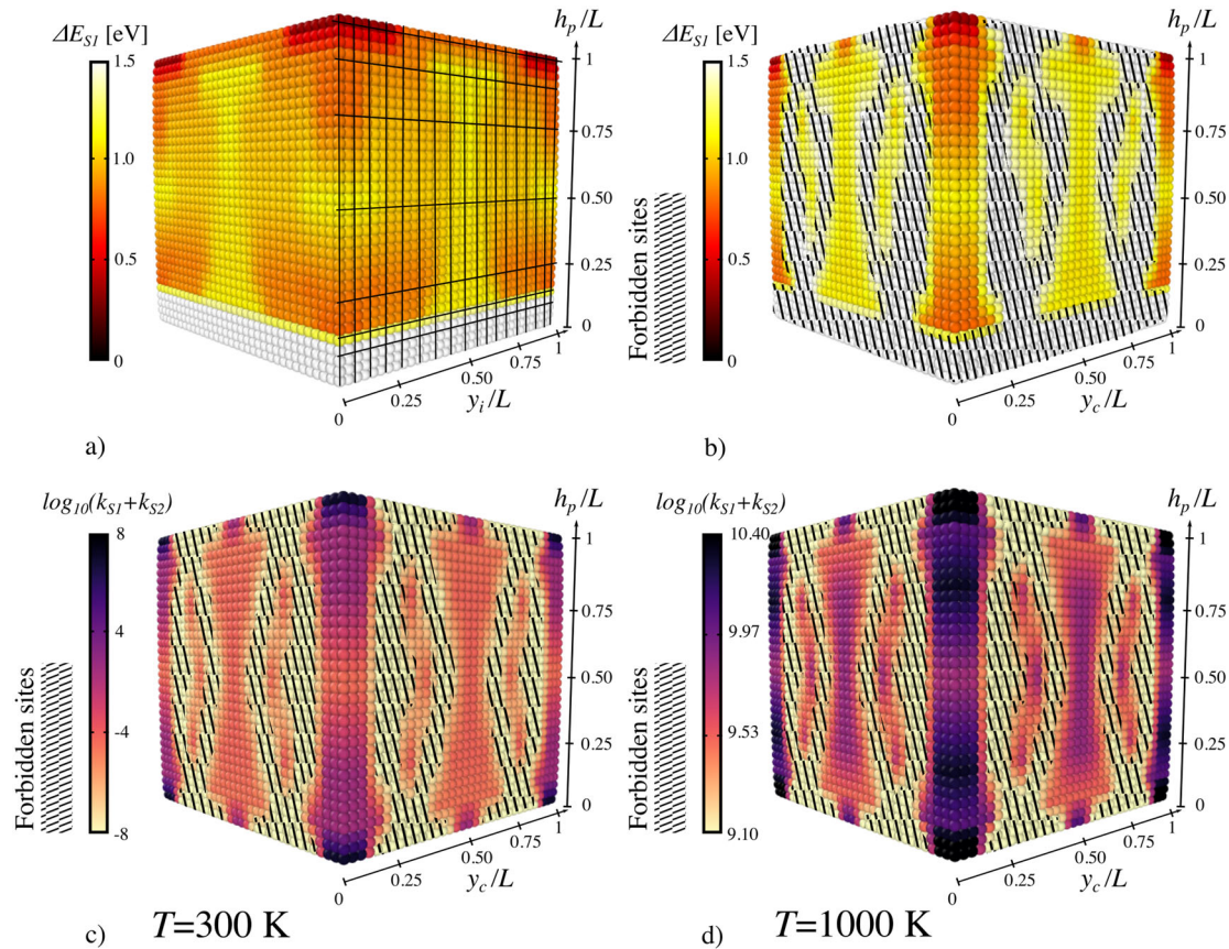
Fig. 4 Mapping of the surface dislocation nucleation energy and rate for an MgO nanocube at \varepsilon = 11\% . a, b show the 0 K activation energy \Delta E as function of the initial and relaxed nucleation centre positions, respectively y_i/L and y_c/L . Both plots consider only one slip system S1 on each face. c, d show the cumulative dislocation nucleation rate \log_{10}(k_{S1} + k_{S2}) calculated using Eq. (1), respectively, at T = 300 and 1000 K. Both orthogonal slip systems S1 and S2 are considered on each face. The black grid shows the NEB calculation mesh. Forbidden sites are marked as hatched domains.
