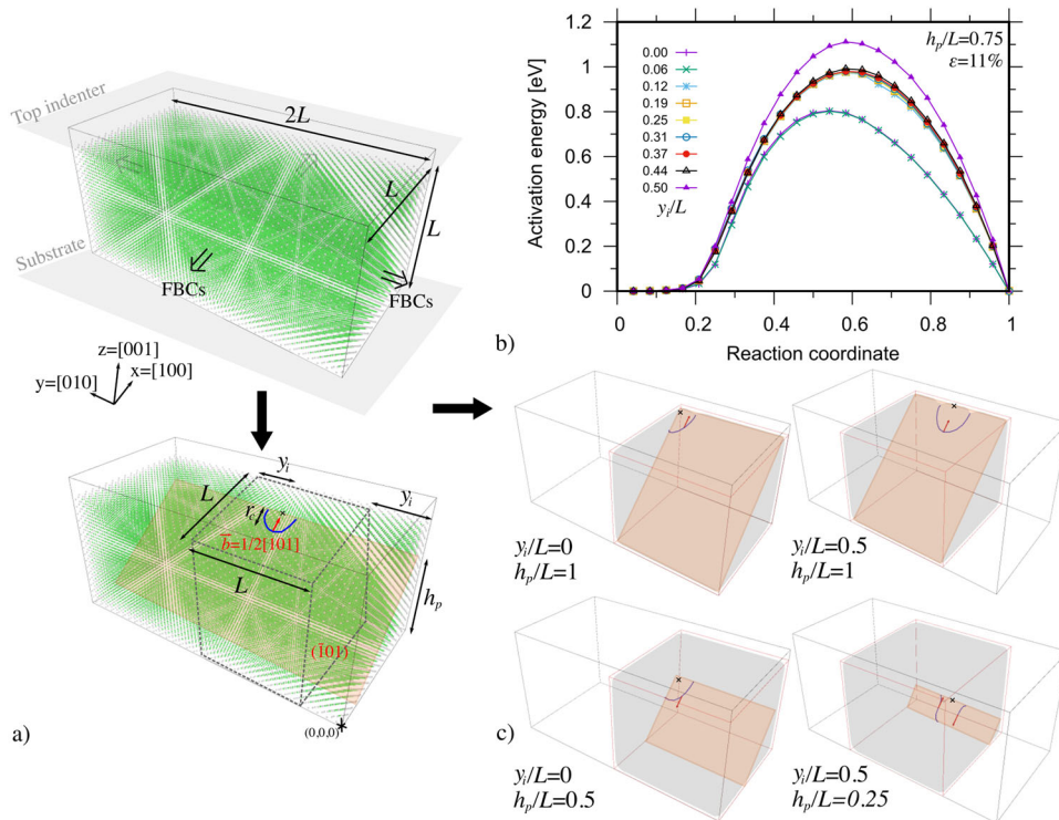
Fig. 2 Modeling surface dislocation nucleation in MgO nanocubes using a multi-step NEB approach. a Illustration of the first NEB step performed on a 2L long MgO nanowire with a square section of edge L constrained by two force fields i.e. the top indenter and the substrate (top image). The saddle point configuration (bottom image) is characterised by a \frac{1}{2}[101](\bar{1}01) dislocation half-loop (line and Burgers vector are shown in blue and red, respectively) emitted at (L, L, h_p) , from the back surface. Only Mg atoms are shown for the sake of clarity (fcc and surface atoms are coloured, respectively, in green and light-grey). The original simulation cell of the nanowire (before loading) is shown using grey-solid lines. The grey-dashed lines refer to a typical nanocube, carved out to compute the site dependence of the surface dislocation nucleation energy barriers during the second NEB step. b Examples of surface dislocation nucleation energy barriers in a nanocube for y_i/L ranging from 0 to 0.5 and h_p/L = 0.75 . c Examples of configurations for dislocation nucleation events from a corner ( y_i/L = 0 , h_p/L = 1 ), from the mid-top edge ( y_i/L = 0.5 , h_p/L = 1 ), the mid-side edge ( y_i/L = 1 , h_p = 0.5 ) and the lower mid-surface region ( y_i/L = 0.5 , h_p/L = 0.25 ).
