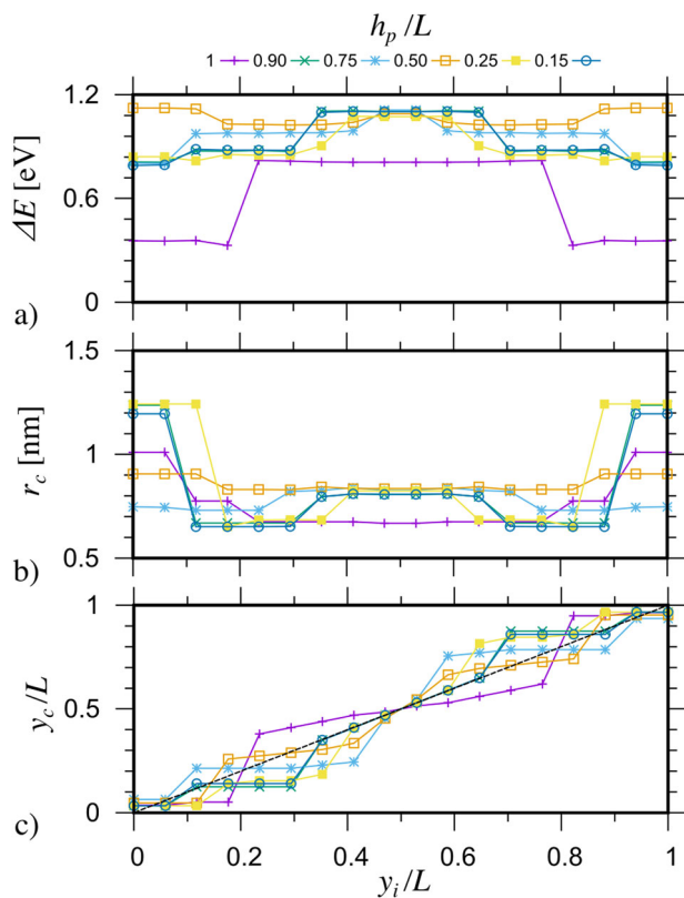
Fig. 3 Side-surface site dependence of dislocation nucleation in a MgO nanocube at \varepsilon = 11\% . a 0 K activation energy \Delta E , b critical dislocation radius r_c and c relaxed position of the nucleation centre y_c/L , as a function of the initial position y_i/L .
