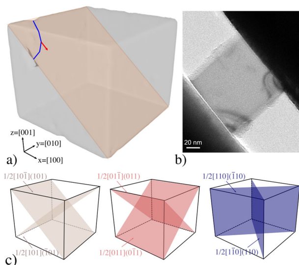
Fig. 1 Surface dislocation nucleation in MgO nanocubes and slip systems. a MgO nanocube compression modeled using MD. A perfect \frac{1}{2}[110]\{110\} dislocation nucleates from a top corner (blue line), just below the indenter. The red arrow refers to the Burgers vector direction. b Surface dislocation nucleation in a MgO nanocube observed during in situ TEM nanocompression test at room temperature (courtesy of Pr. Masenelli-Varlot). c \frac{1}{2}[110]\{110\} slip systems in MgO.
