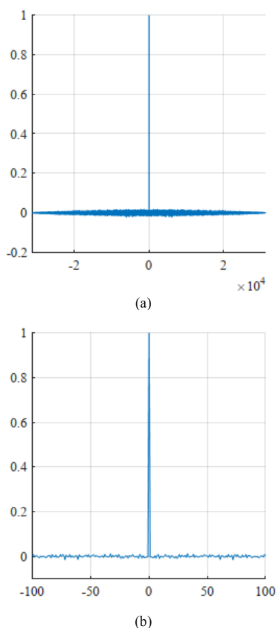
Figure 10. (a) Auto-correlation of sequence X ; (b) A zoom of the auto-correlation of sequence X
